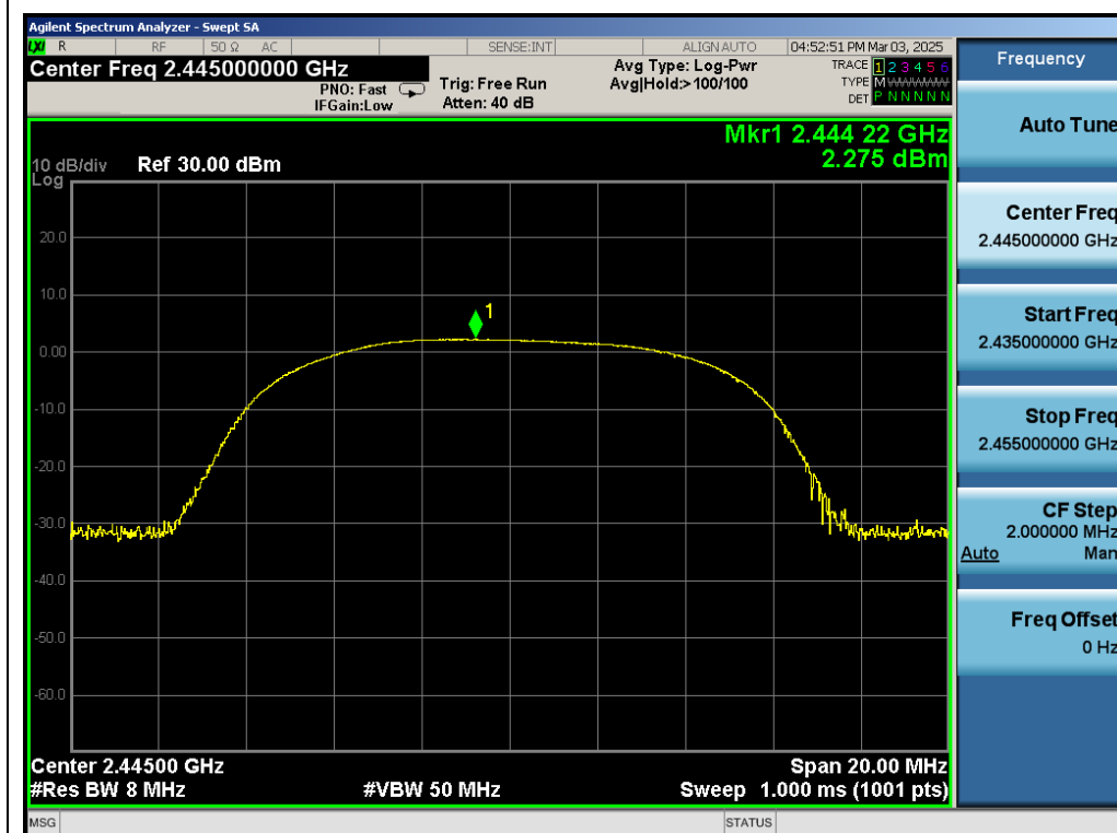
Test_Graph_GFSK_ANT1_2445_Peak Power
