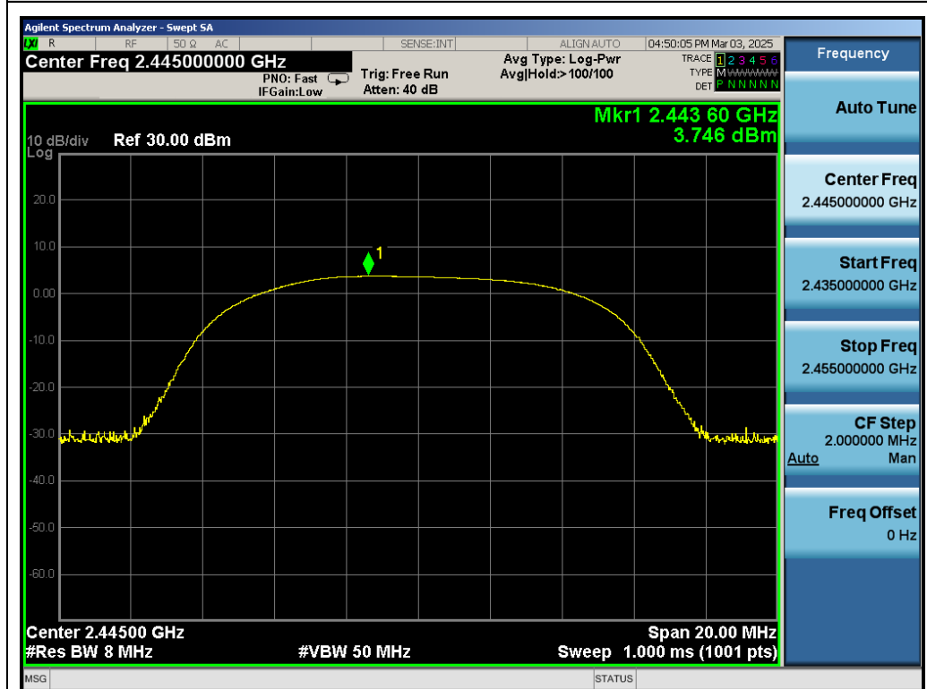
Test_Graph_GFSK_ANT1_2445_Peak Power
