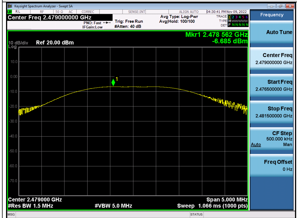
Test_Graph_2.4G_ANT1_2479_Peak Power
