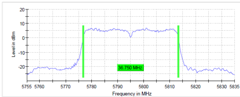
99 % Bandwidth
