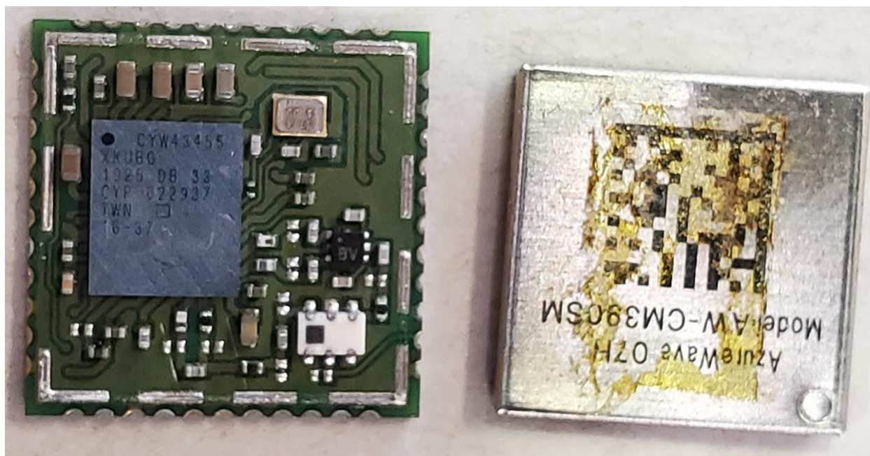
View of wifi chip without shielding
