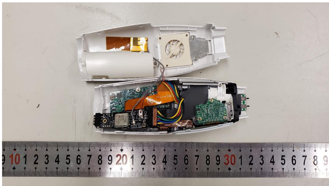
Internal view of handpiece (with heat-sink being removed)
