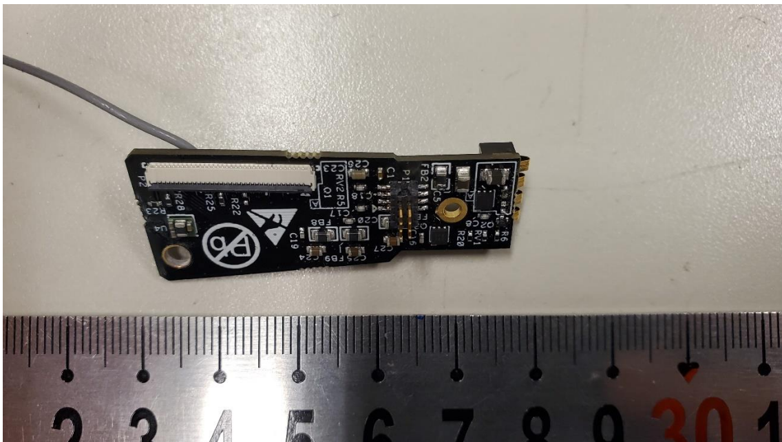
View of wifi module
