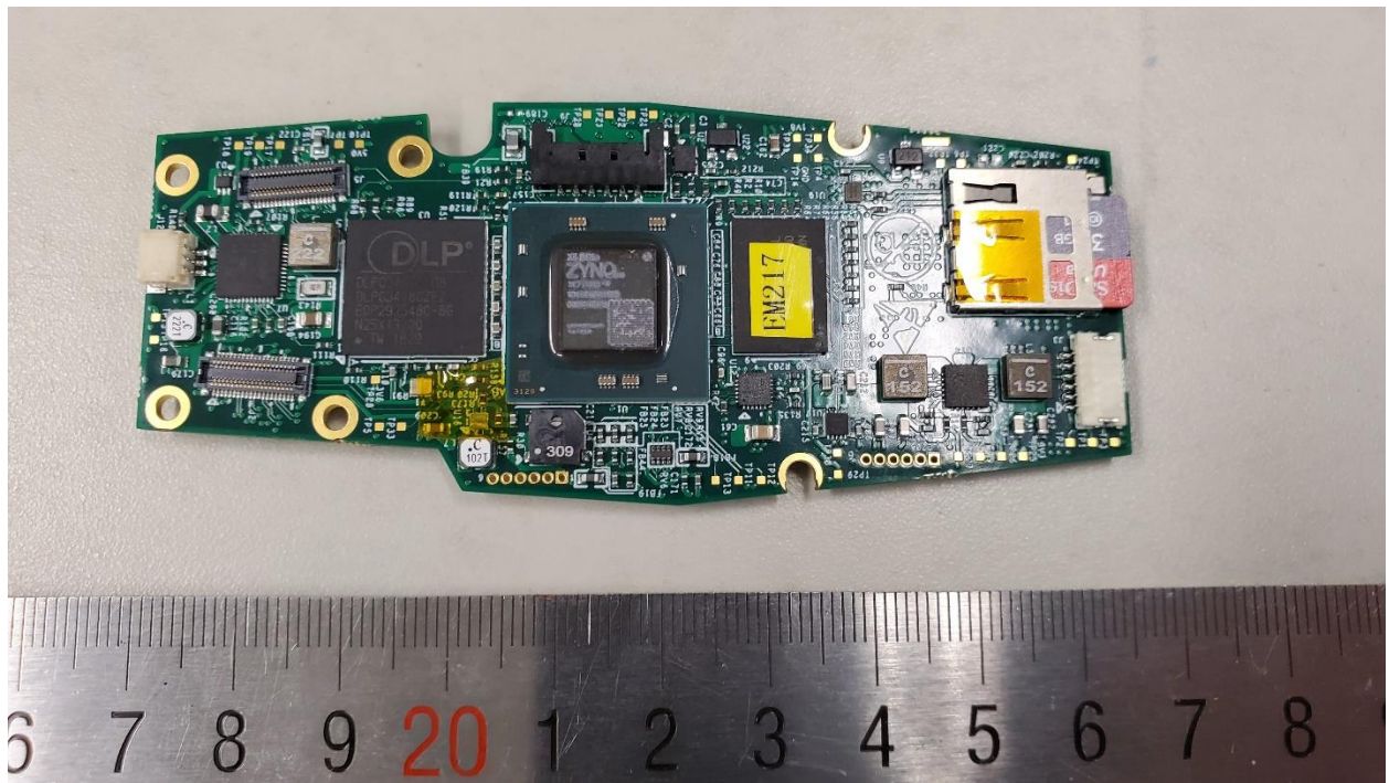
Internal view of PCB
