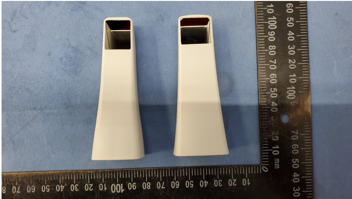
View of the tips
