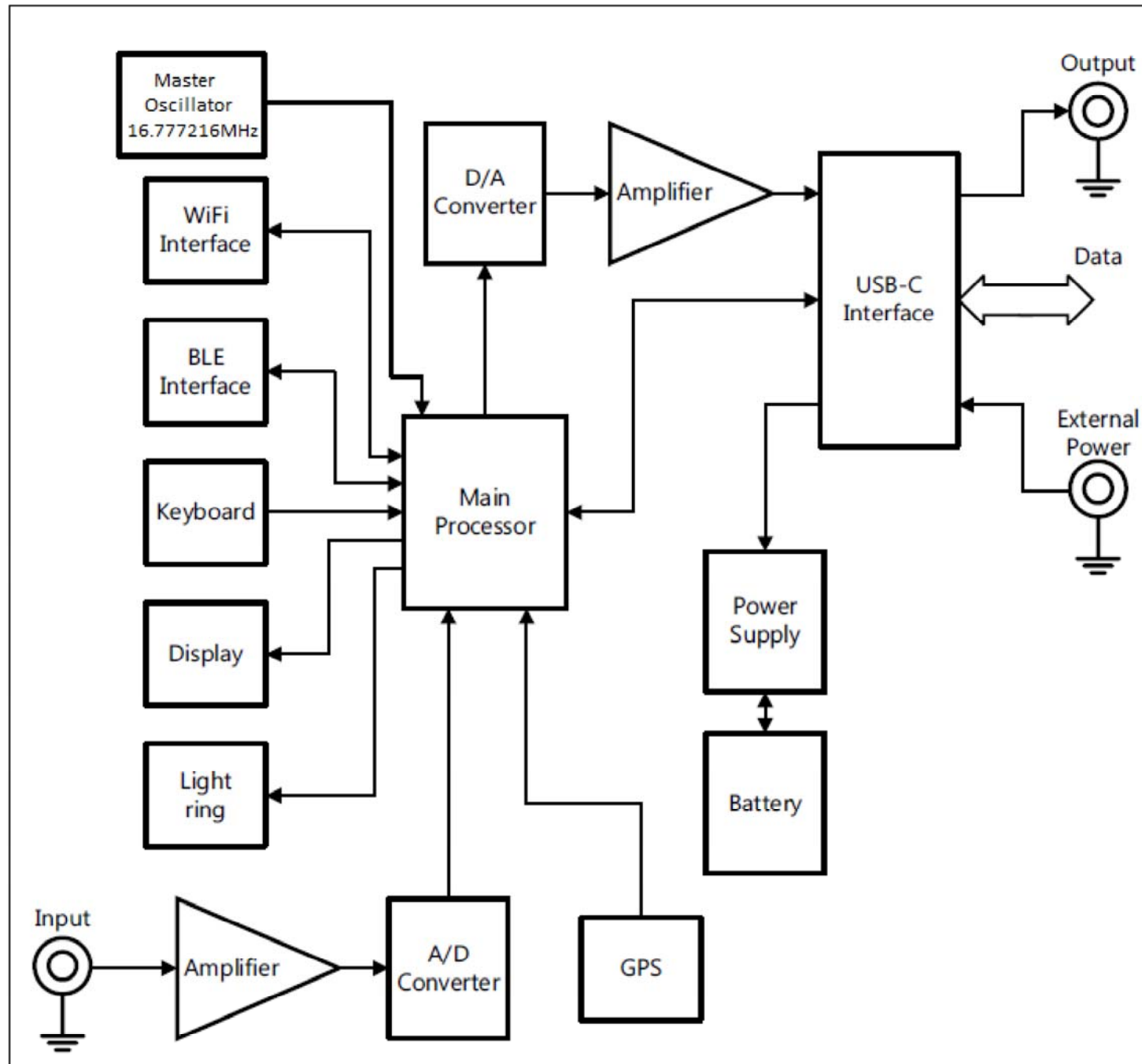
Fig. 1.2 Block diagram of Type 2255
