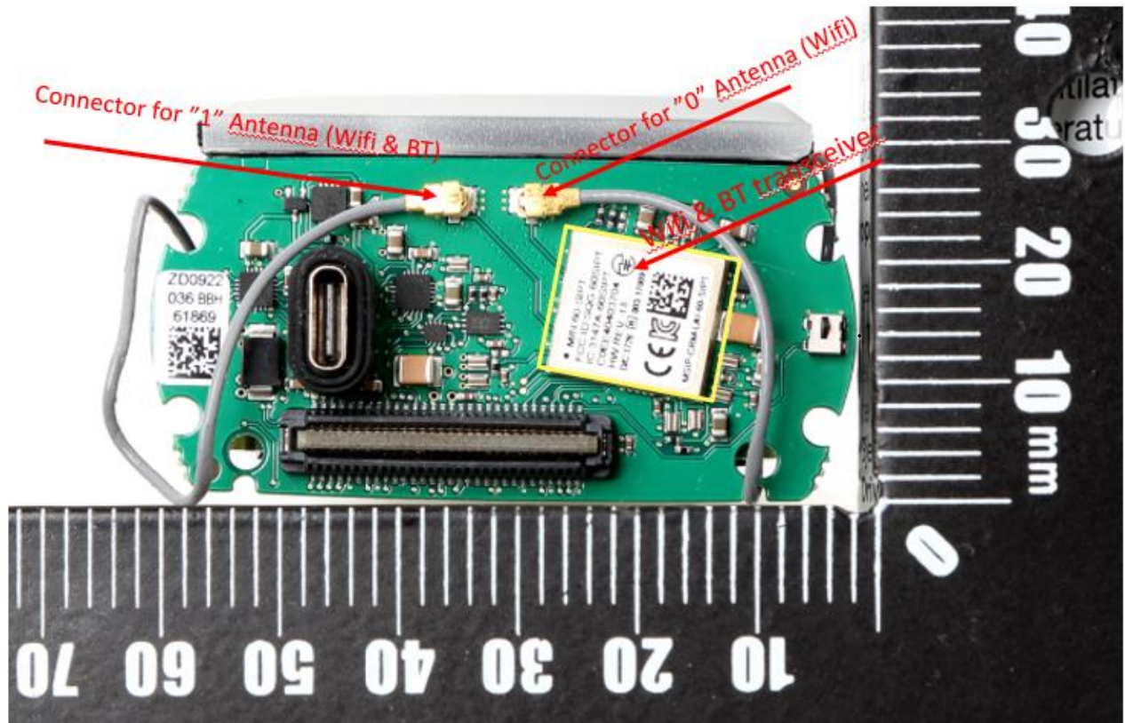
Interface PCB (ZD0922) – USB interface and radio transmitter
