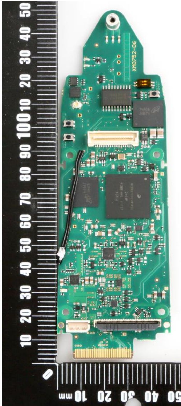
ZD0920 – Digital PCB. (CPU, RAM, FLASH etc.) Frontside.
