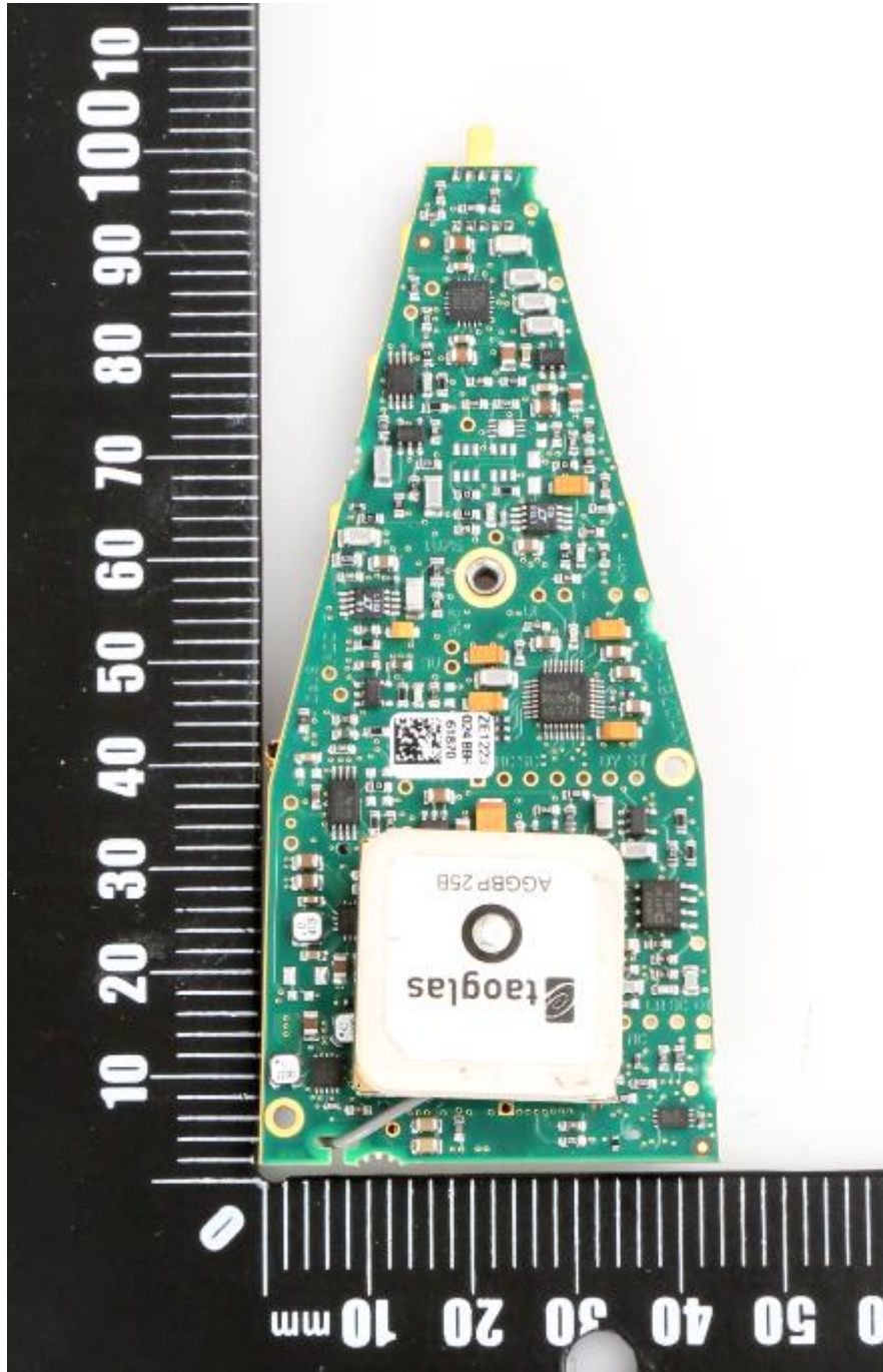
ZE1223 – Analog PCB, Placement of GPS antenna. Top side
