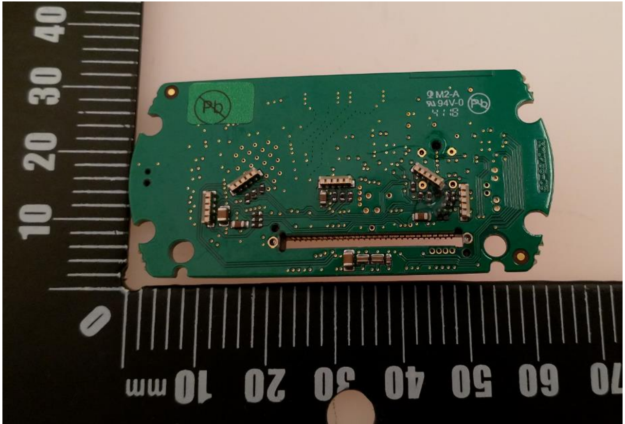
Interface PCB (ZD0922) – USB interface, radio transmitter, and LED's for lighting (Back)
