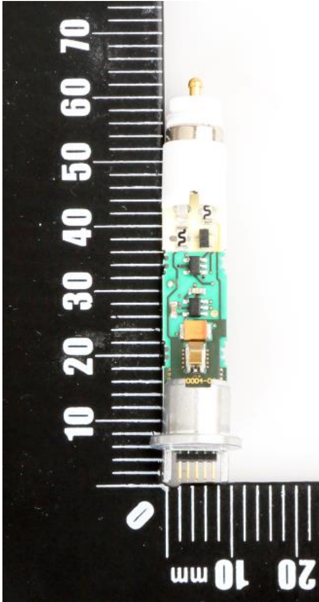
ZC0040 – Preamplifier. Front side
