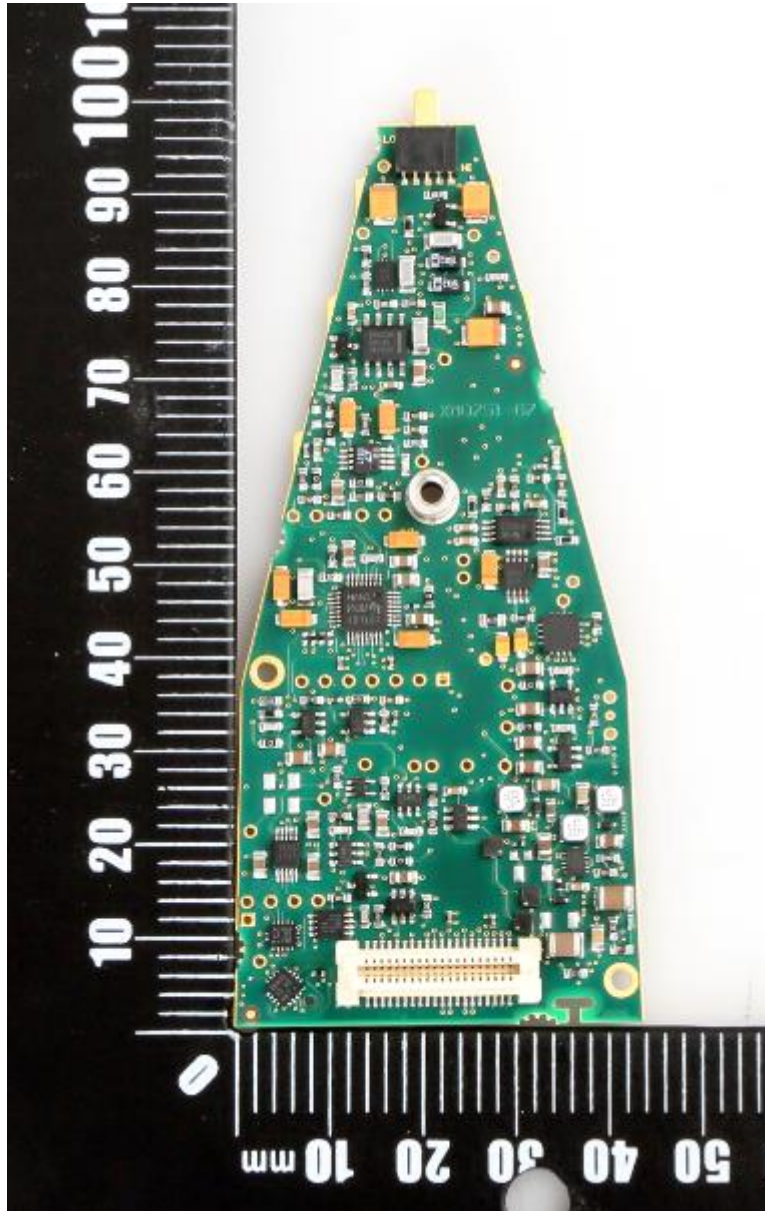
ZE1223 – Analog PCB. Bottom side
