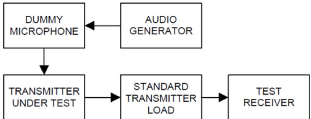
Figure 7.8.1 Modulation limiting test setup
