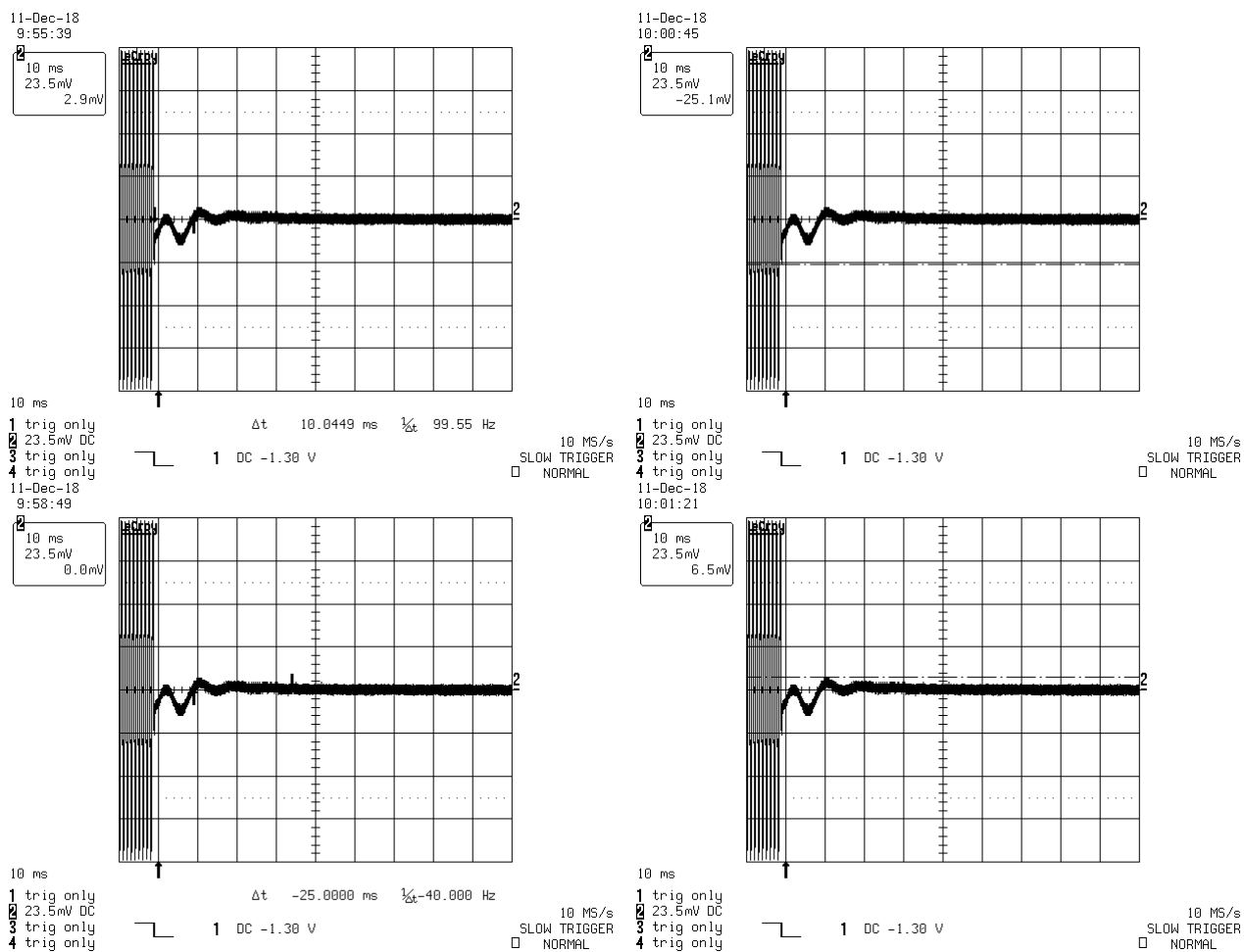
Plot 7.7.1 Transient frequency behavior during power ON test results at low carrier frequency
