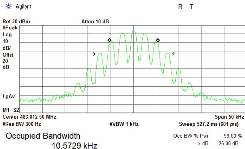
Plot 7.2.2 Occupied bandwidth test result at 483.0125 MHz with Private Line
