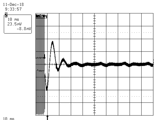
Plot 7.7.3 Transient frequency behavior during power ON test results at high carrier frequency
