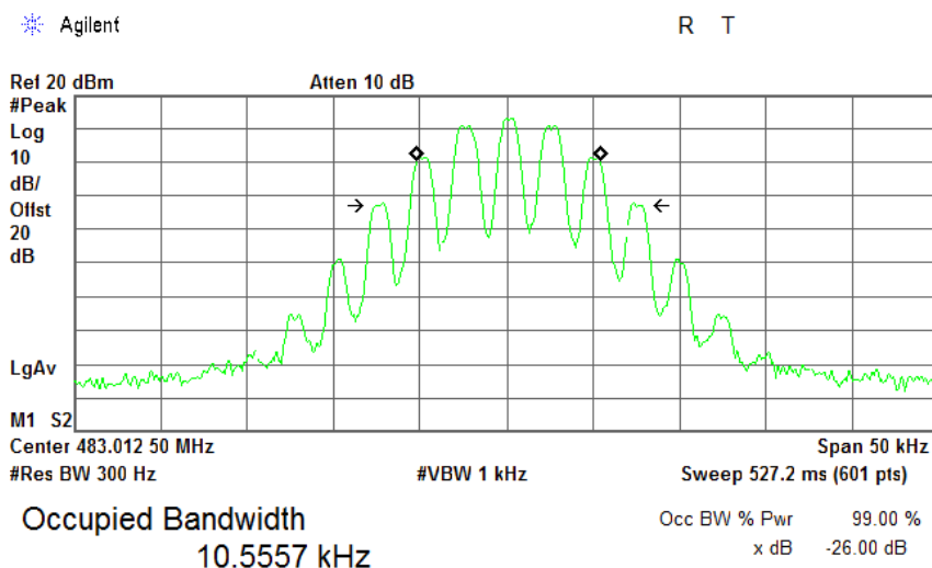
Plot 7.2.1 Occupied bandwidth test result at 483.0125 MHz
