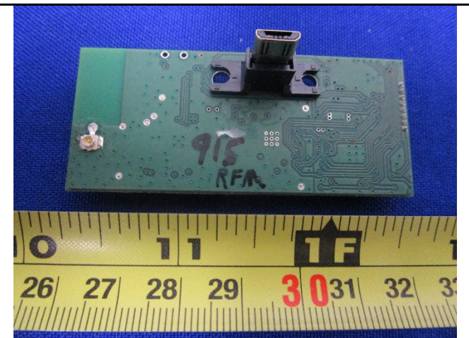
RF Module - Bottom View
