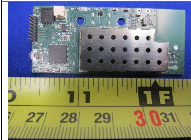
RF Module - Top View
