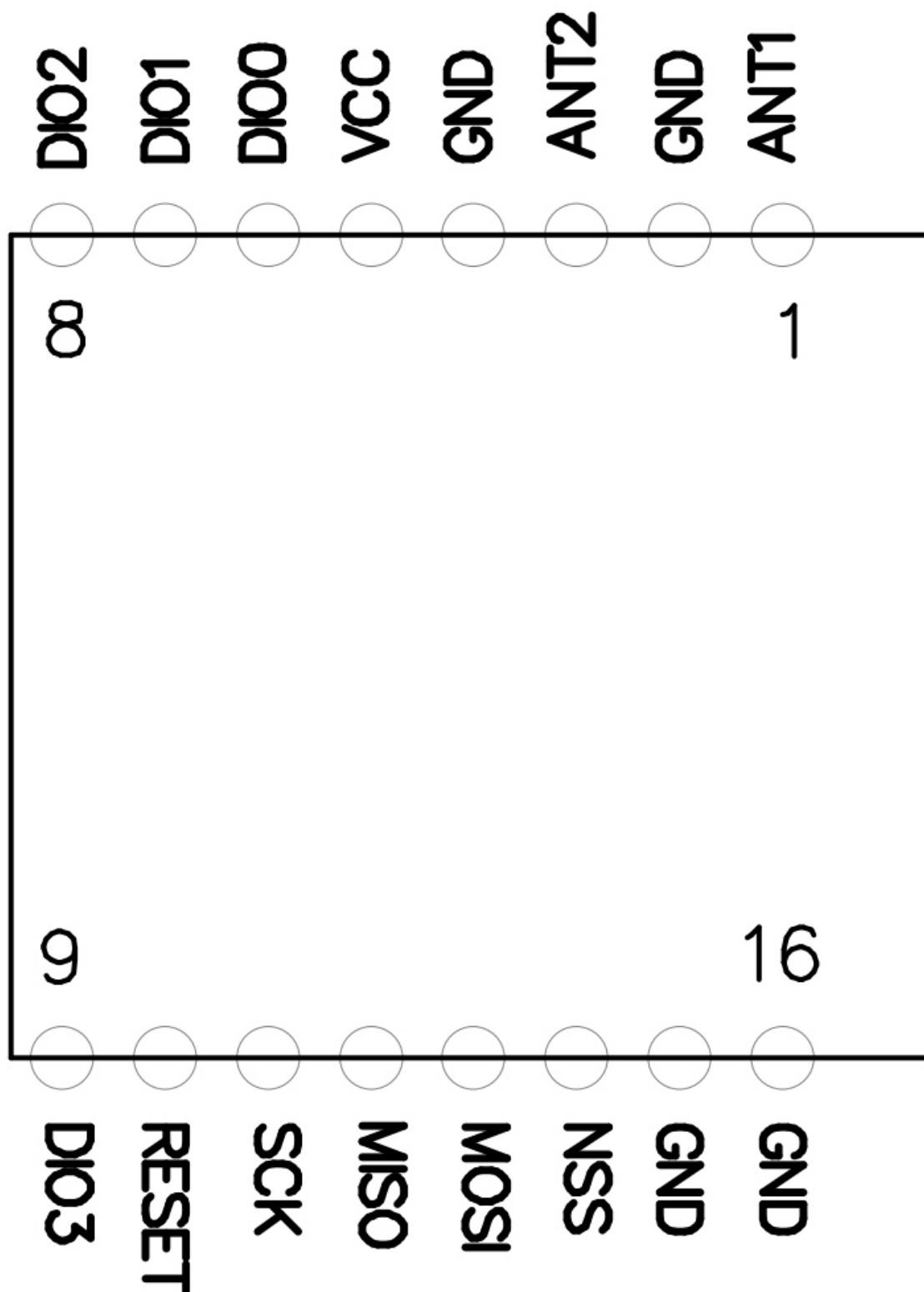
Pic1. TOP View of HPNI01
