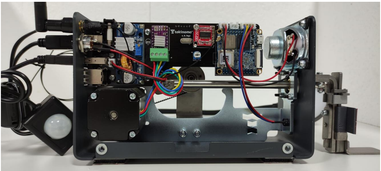
Left view
