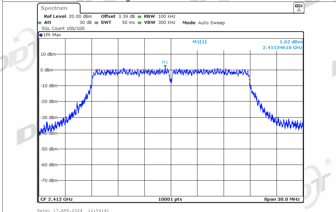
Band Edge NVNT n20 2412MHz Ant1 Emission
