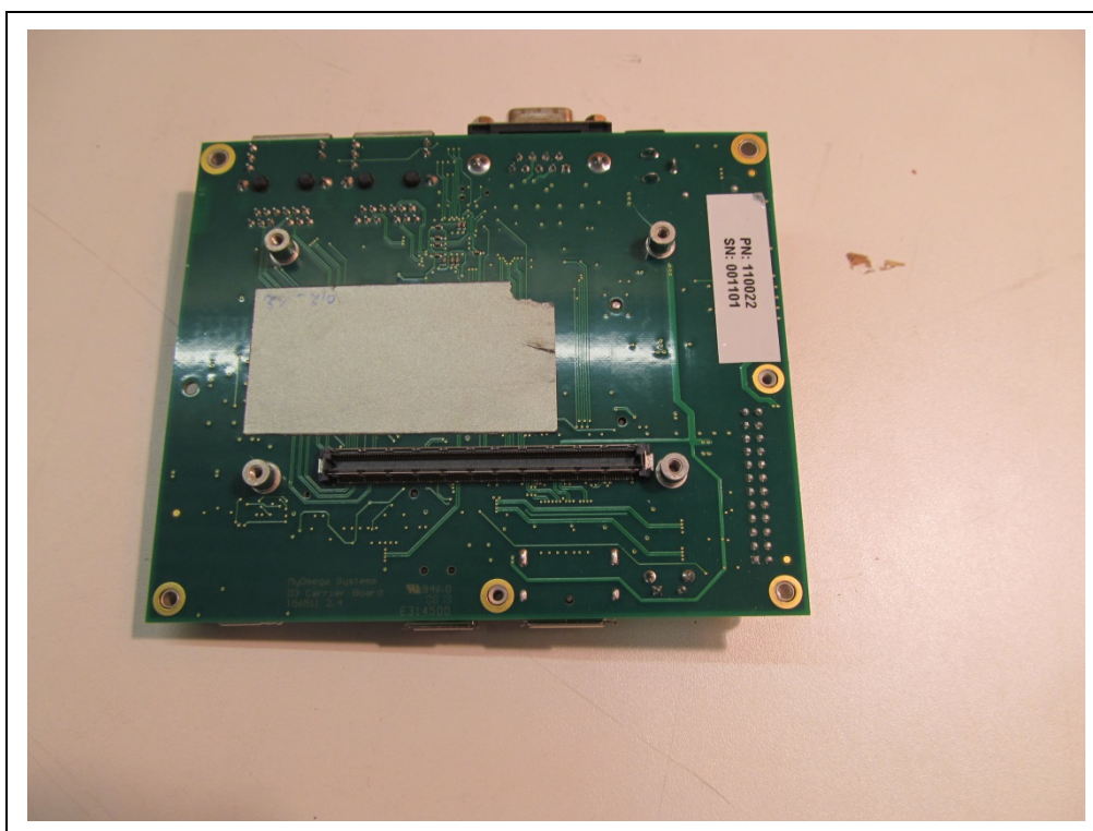
Photograph A3-6: D3 Carrier Board Bottom with adhesive shielding material
