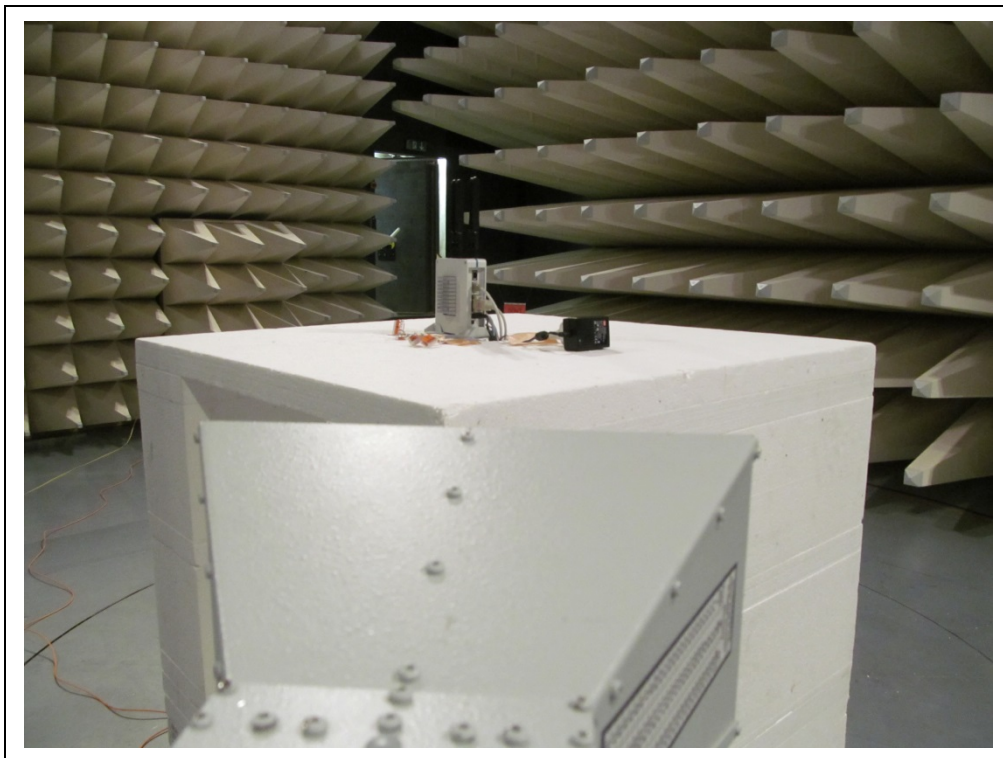
Photograph A1-4: Radiated emissions 6 – 15 GHz at 1 m distance
