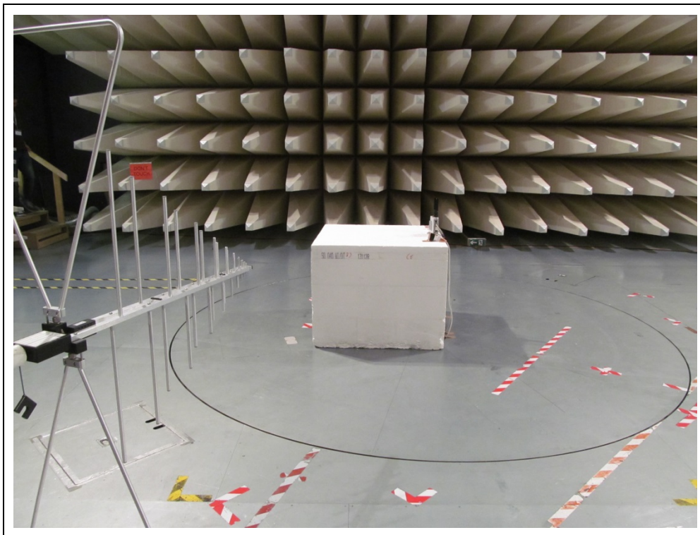
Photograph A1-2: Radiated emissions 30 – 1000 MHz at 3 m distance
