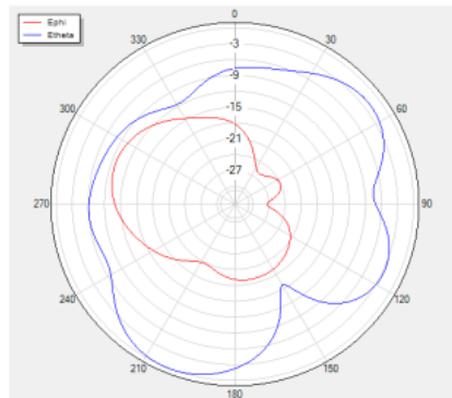
Theta=90 freq=1730MHz
