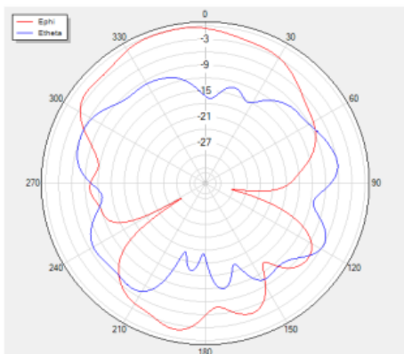
Phi=90 freq=2100MHz
