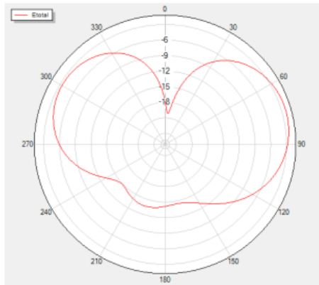
Theta=90 Freq=850MHz
