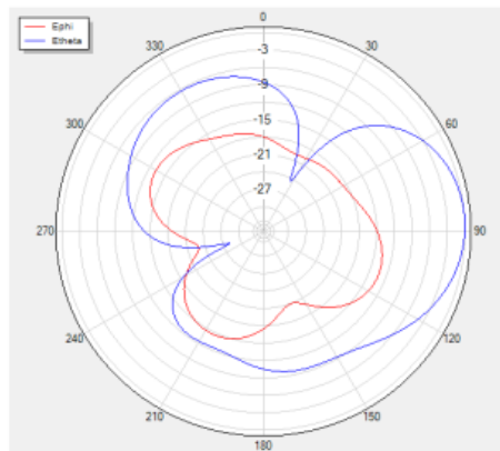
Theta=90 freq=910MHz
