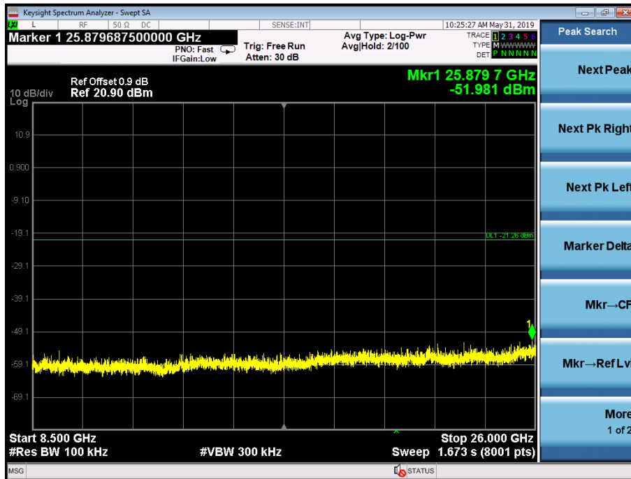
RF Conducted Spurious Emissions_BLE_2440_Ant1
