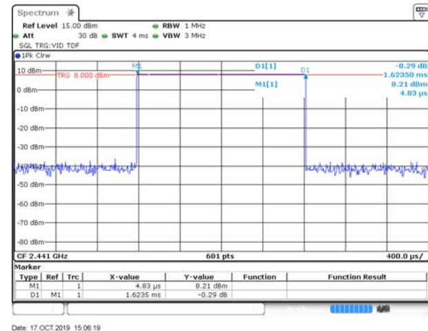
GFSK DH3
