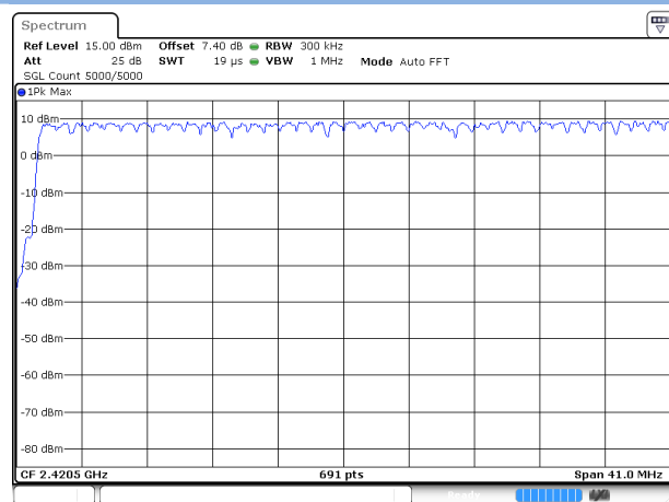
Π/4-DQPSK 2.4 GHz ~ 2.4415 GHz
