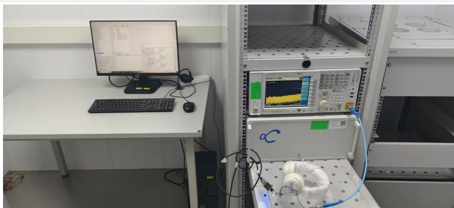
Conducted Test-BLE
