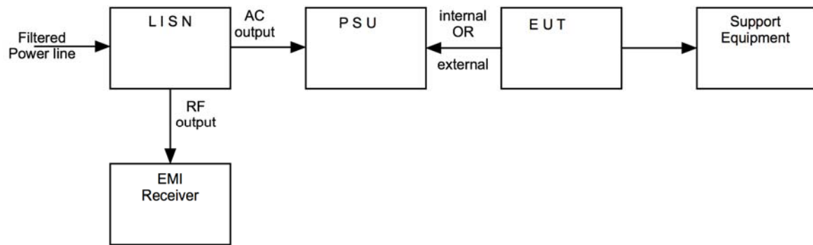
Figure iii Test Setup
