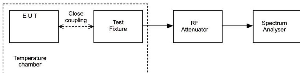
Figure vi Test Setup
