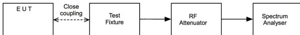
Figure iv Test Setup
