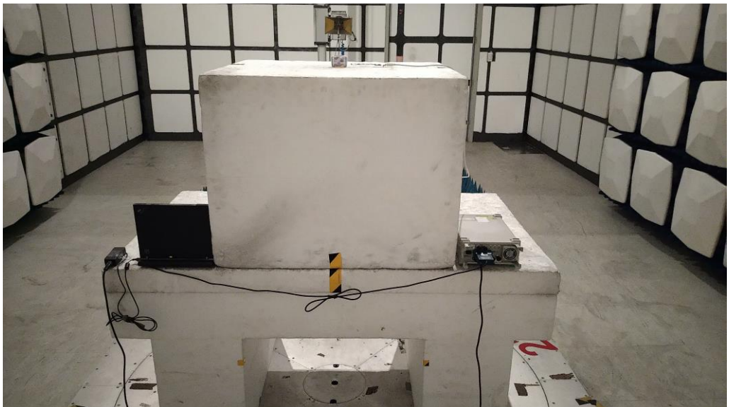
Rear View
