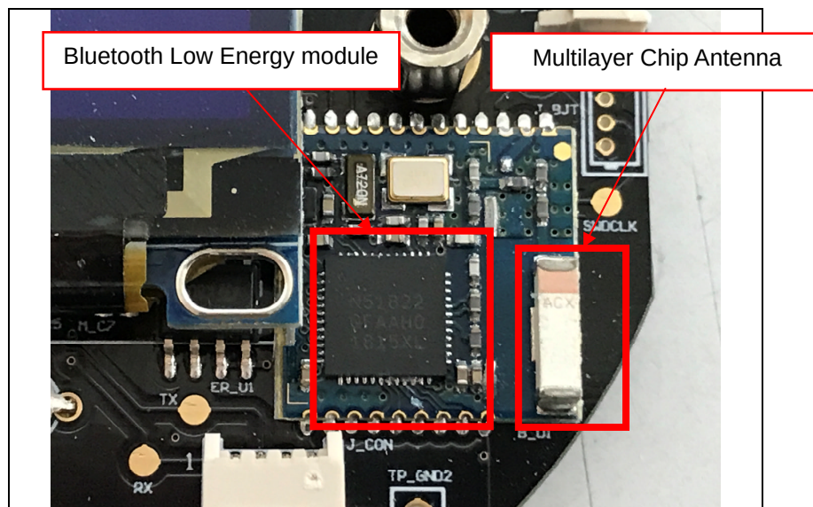
View of Bluetooth Low Energy Module, Antenna
