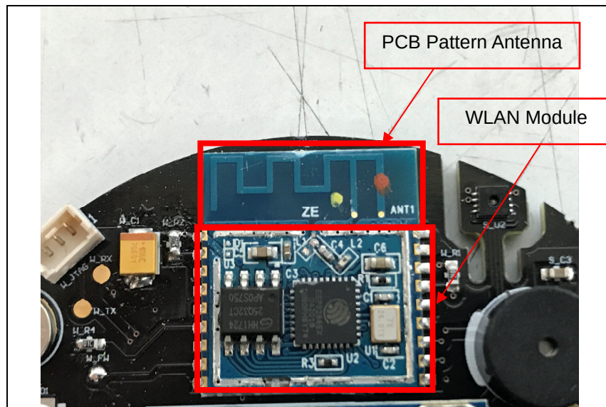
View of WLAN Module, Antenna
