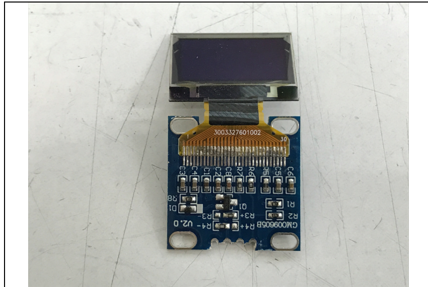
Top view of Sub PCB
