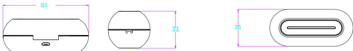
Charging box
