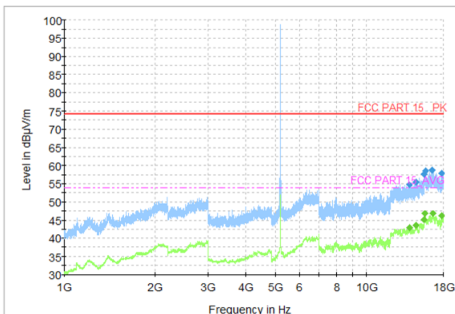
Fig. 73 Transmitter Spurious Emission (802.11a, CH40 5200MHz)
