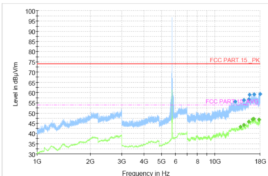
Fig. 97 Transmitter Spurious Emission (802.11ac-VHT80, CH156 5775MHz)
