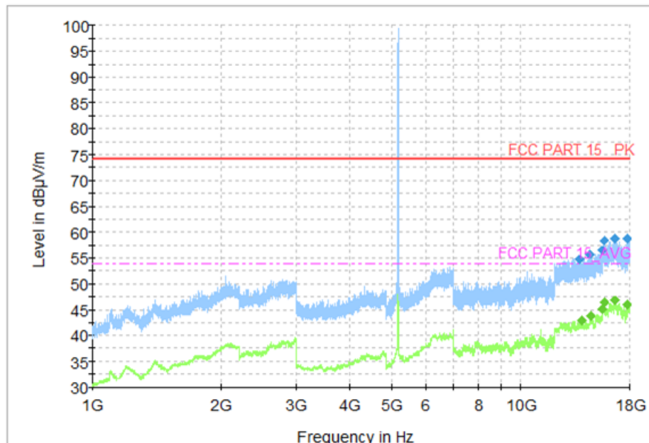
Fig. 72 Transmitter Spurious Emission (802.11a, CH36 5180MHz)
