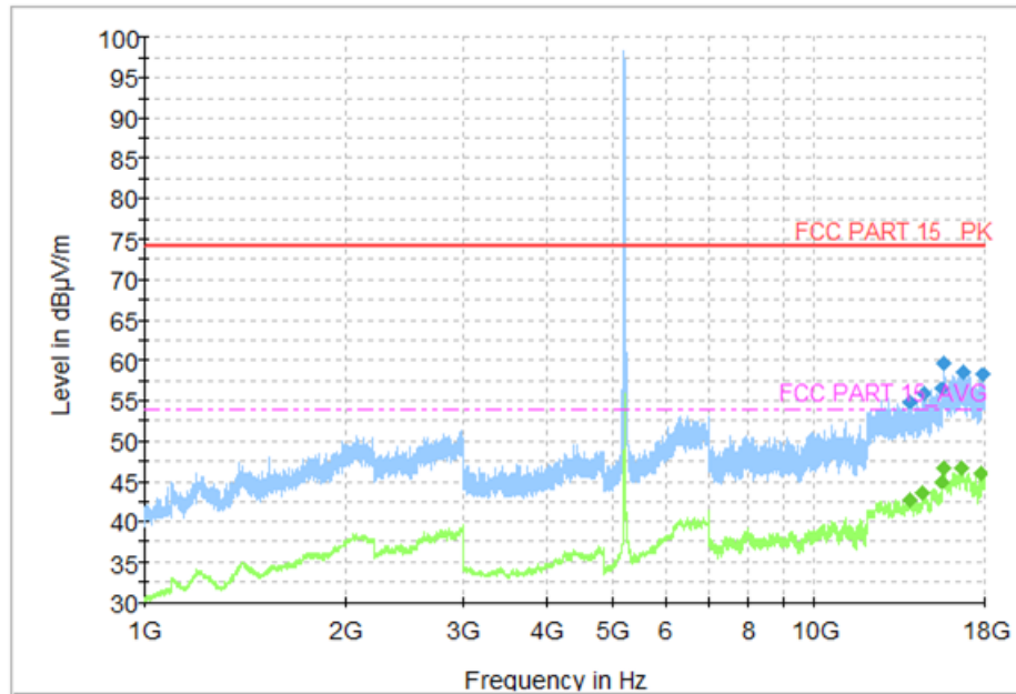
Fig. 85 Transmitter Spurious Emission (802.11n-HT40, CH46 5230MHz)
