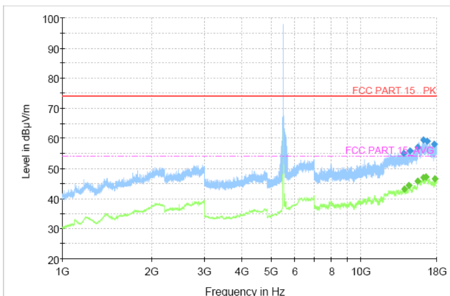
Fig. 95 Transmitter Spurious Emission (802. 11ac-VHT80, CH106 5530MHz)
