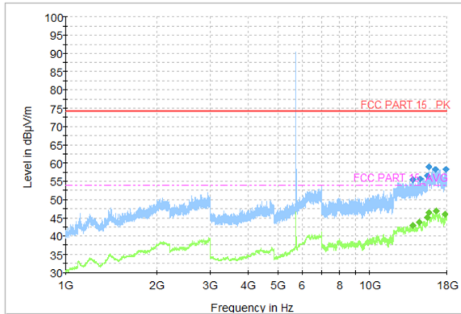
Fig. 81 Transmitter Spurious Emission (802. 11a, CH149 5745MHz)
