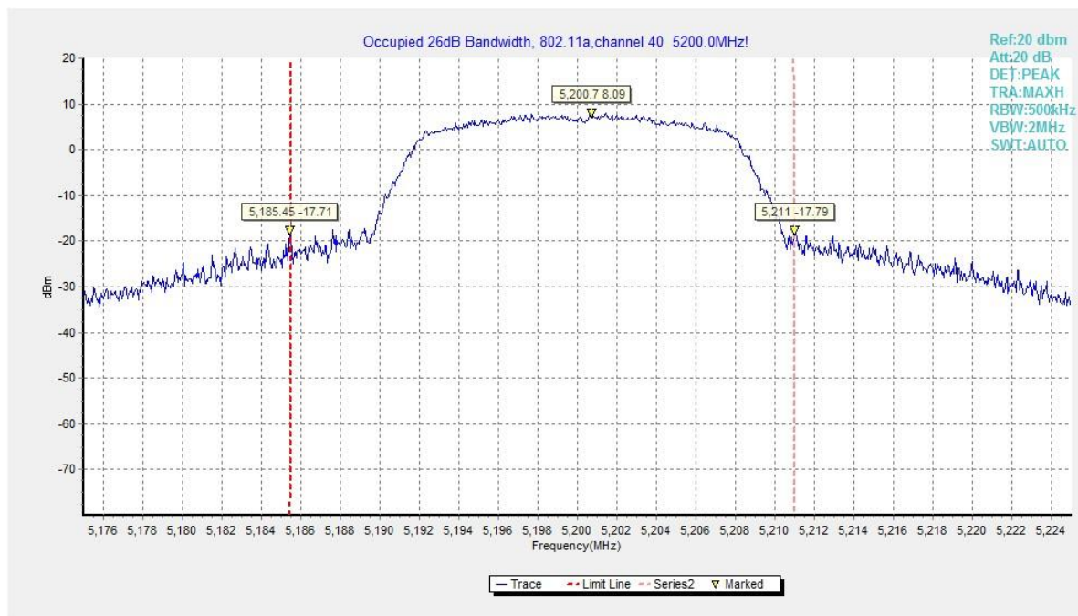
Fig. 11 Occupied 26dB Bandwidth (802.11a, 5200MHz)
