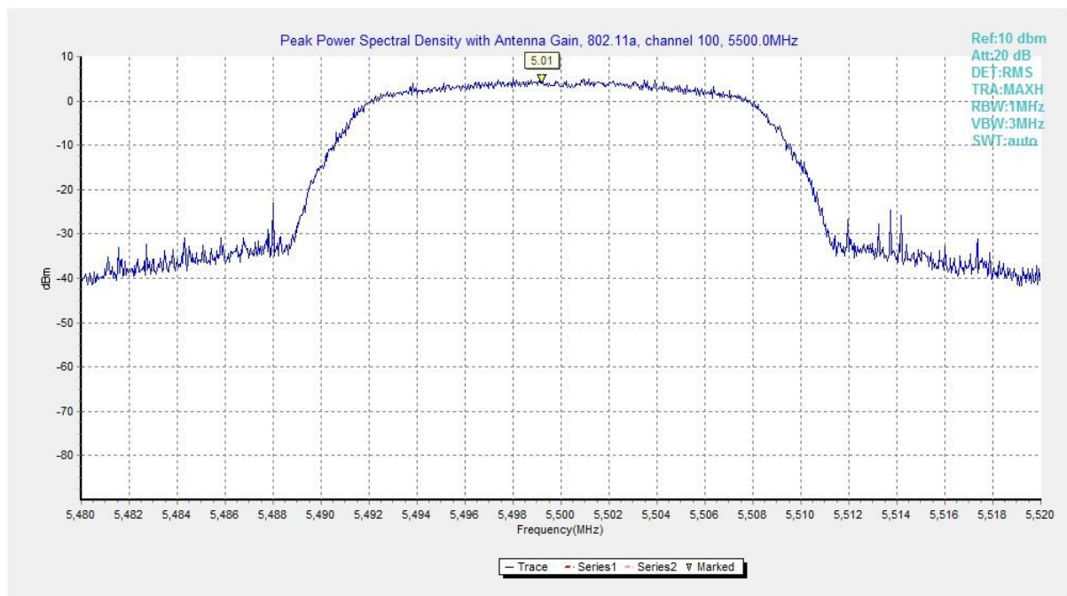
Fig. 7 Power Spectral Density (802.11a, 5500MHz)
