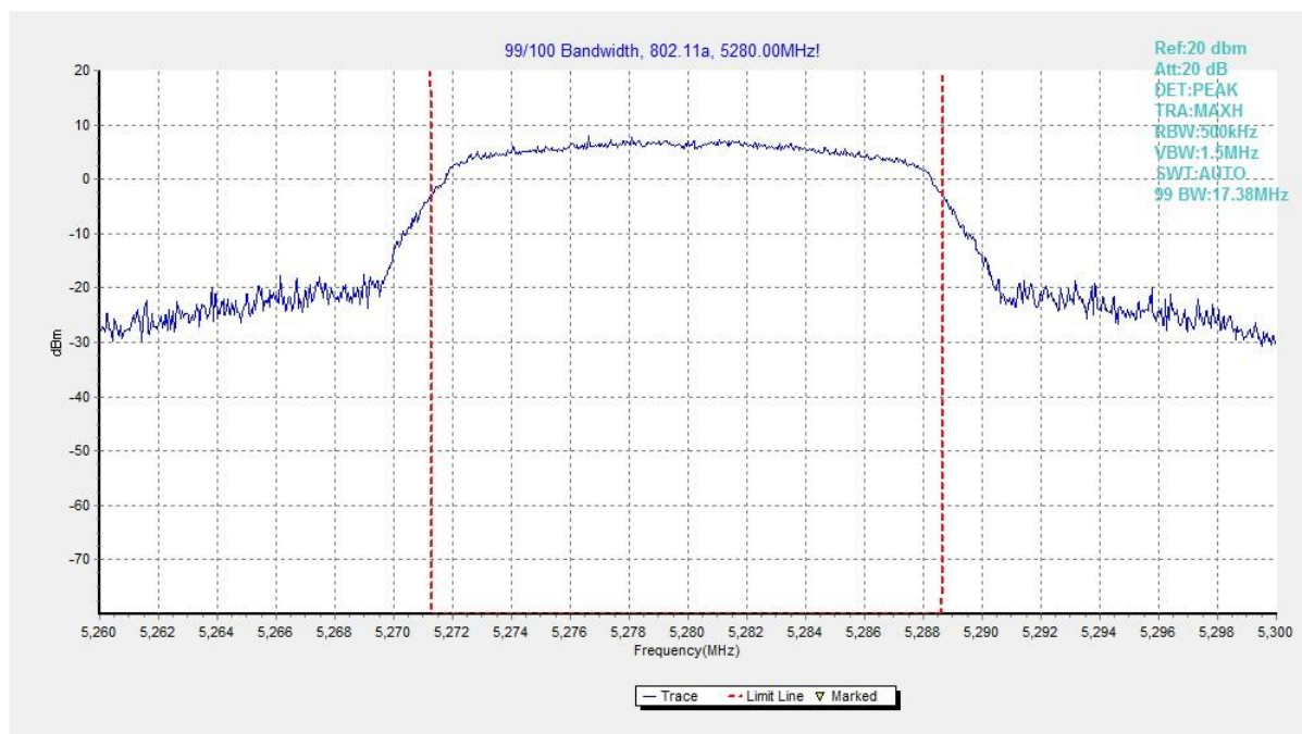
Fig. 40 99% Occupied Bandwidth (802.11a, 5280MHz)
