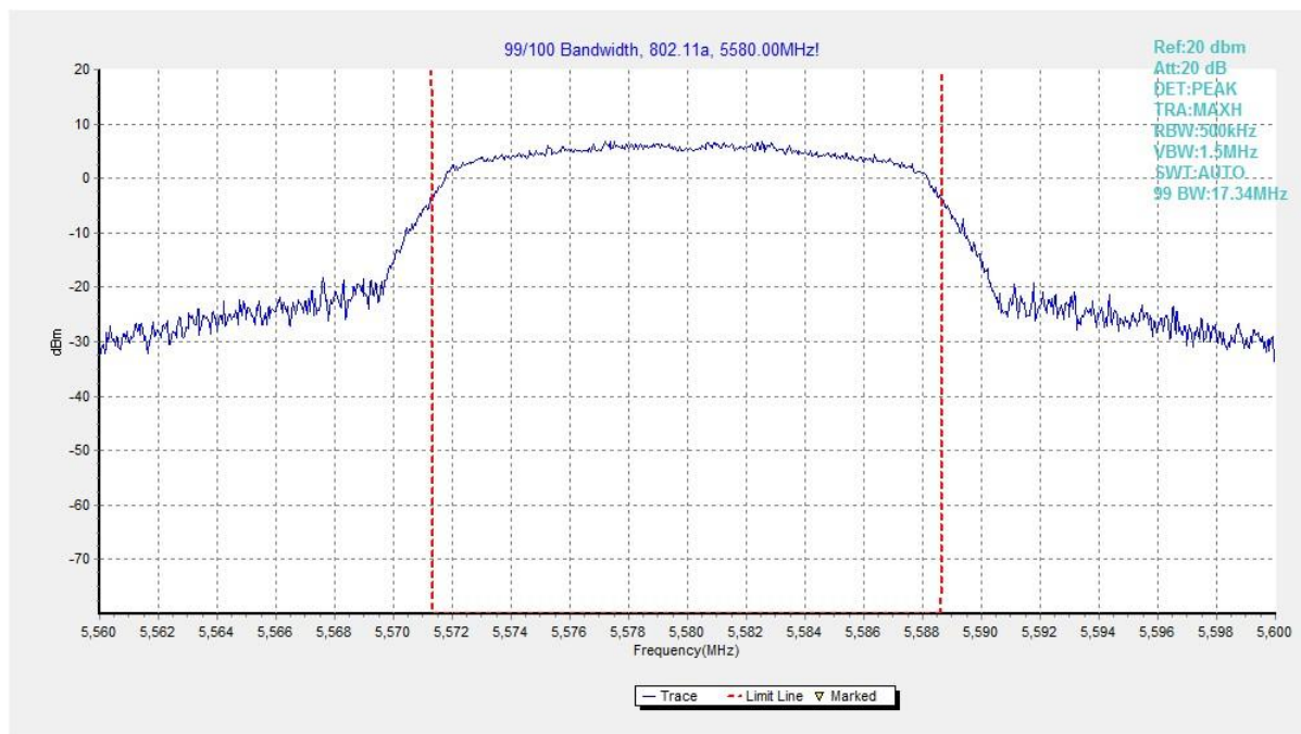
Fig. 43 99% Occupied Bandwidth (802. 11a, 5580MHz)
