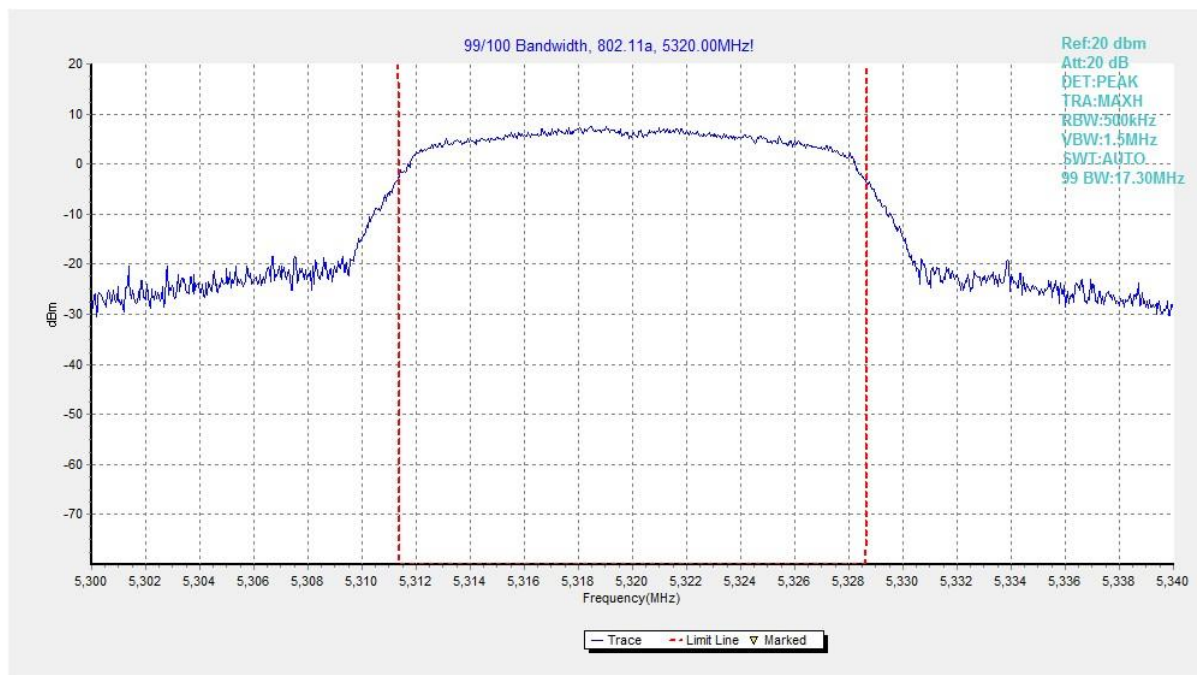
Fig. 41 99% Occupied Bandwidth (802.11a, 5320MHz)
