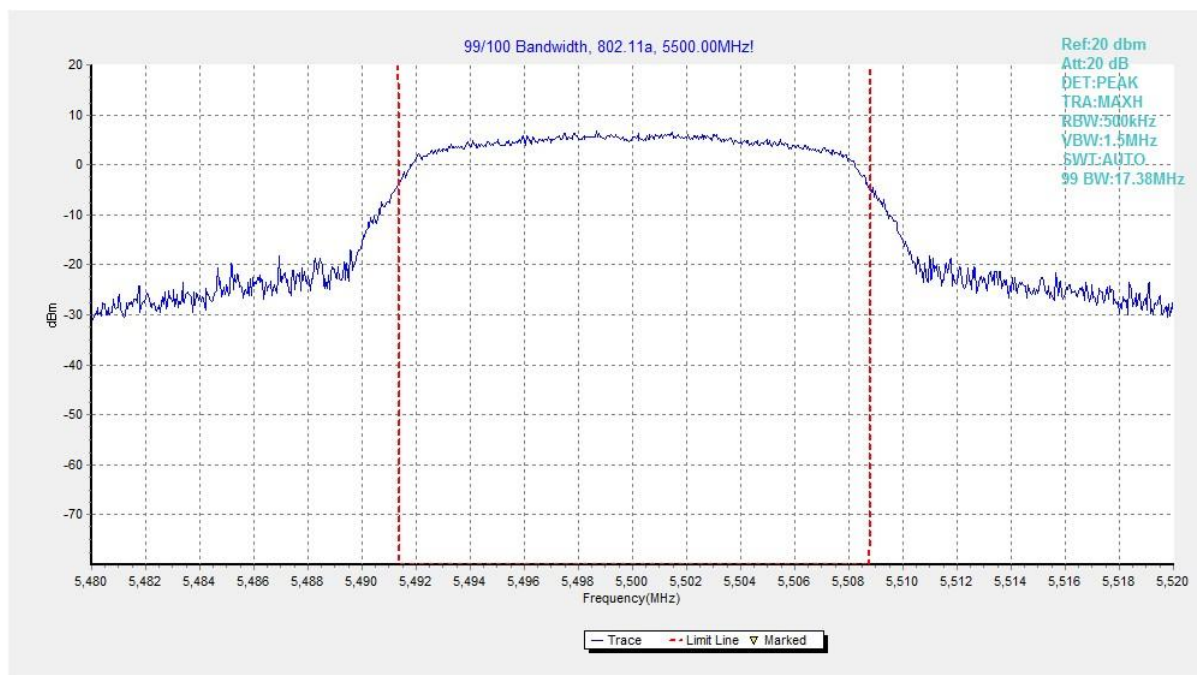
Fig. 42 99% Occupied Bandwidth (802. 11a, 5500MHz)
