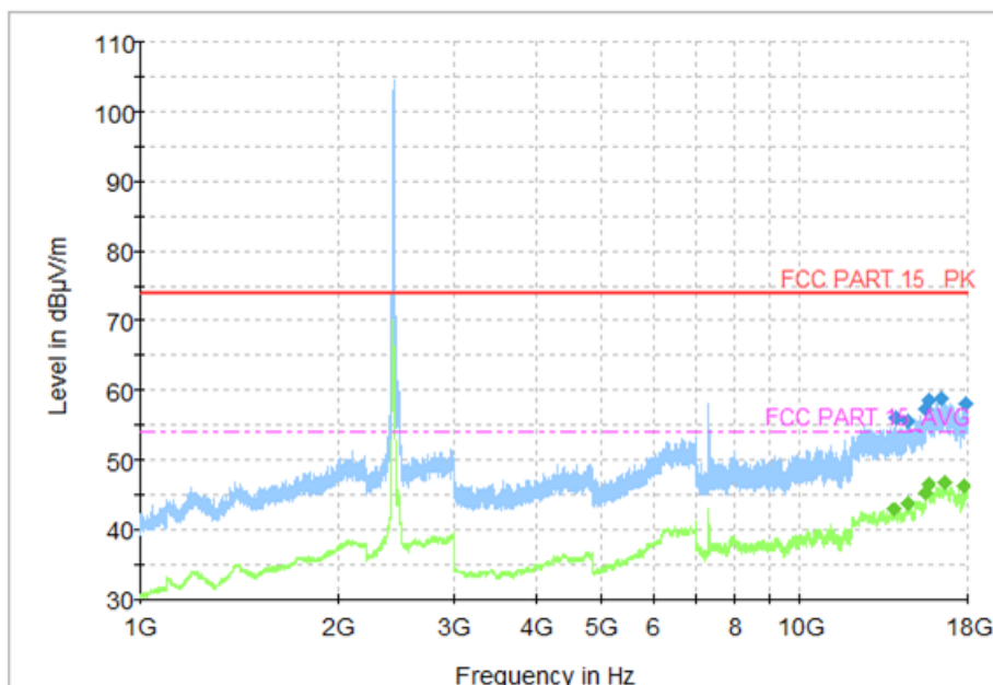
Fig.61 Radiated Spurious Emission (802.11n HT40, CH6, 1 GHz-18 GHz)
