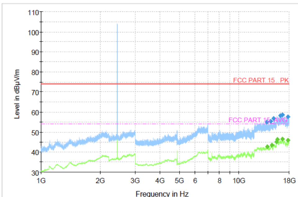
Fig. 43 Radiated Spurious Emission (GFSK, Ch39, 1 GHz ~18 GHz)
