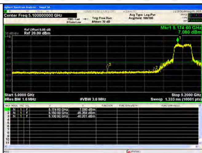
802.11n(HT40)-5190
