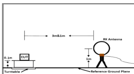
Below 30MHz
