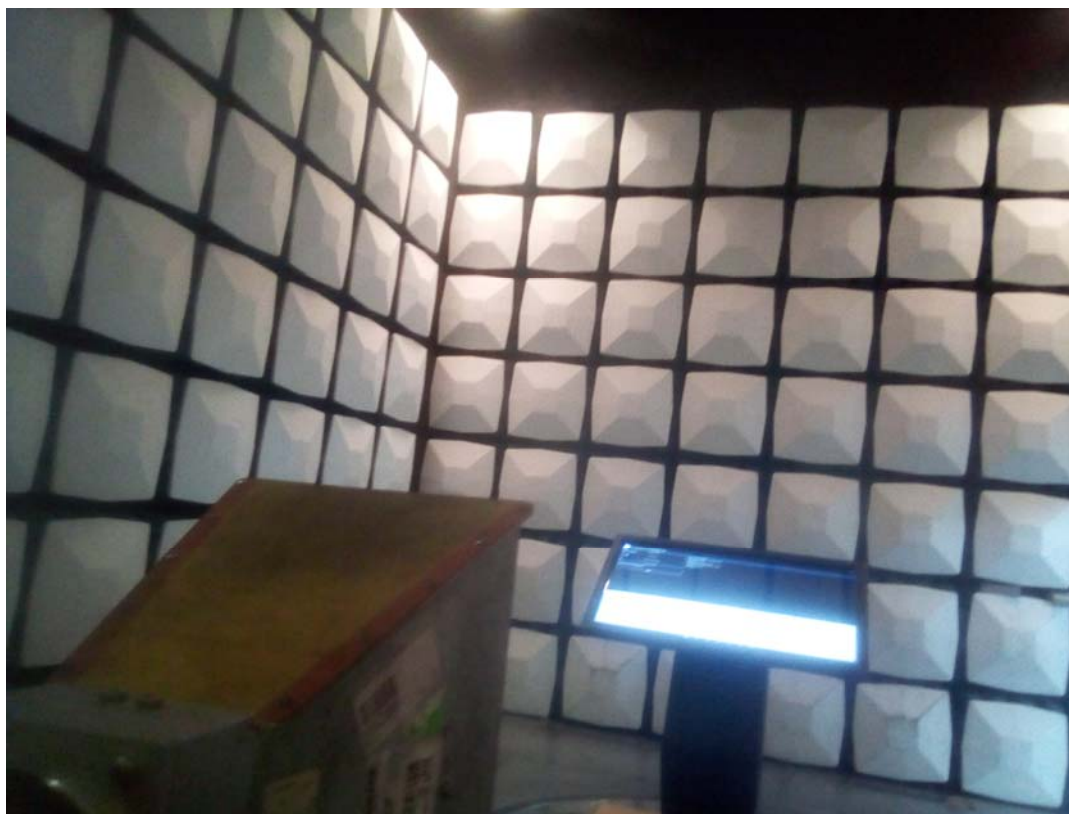
Radiated Emission Above 1GHz View DGSNKTCH43BK
