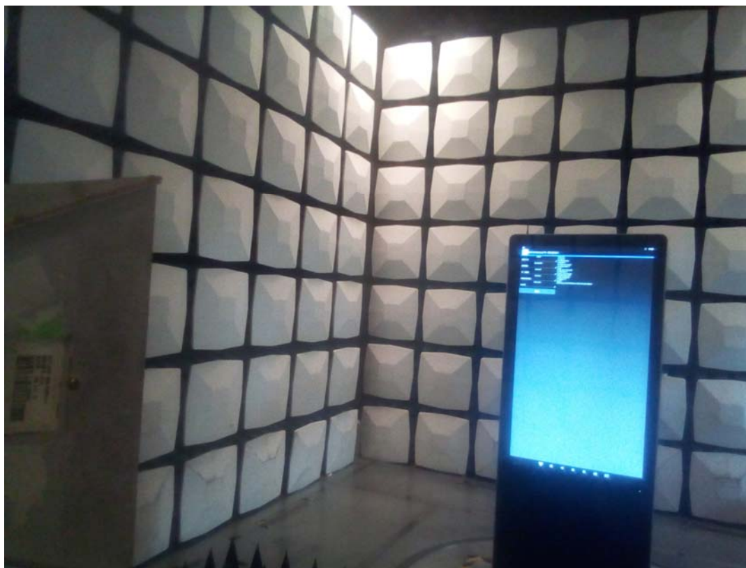
Radiated Emission Above 1GHz View DGSNFSTCH43
