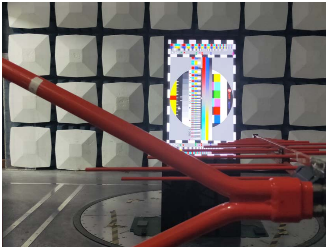
Radiated Emission Above 1GHz View DGSNAFNT43
