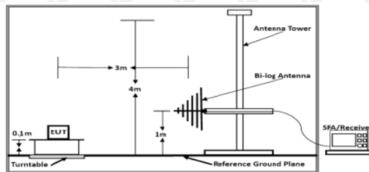
Figure 2. 30MHz to 1GHz
