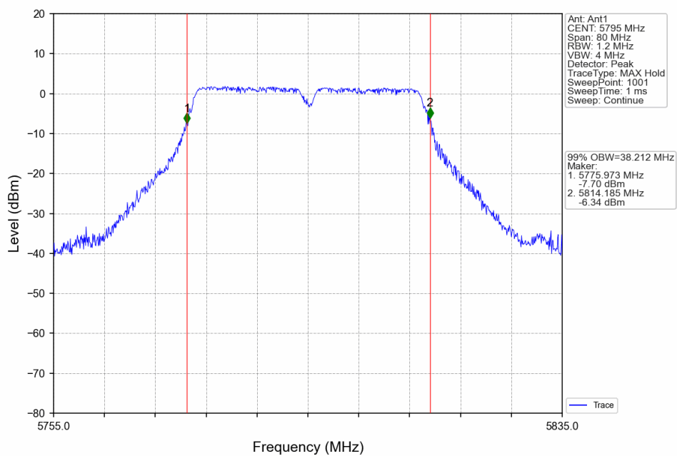
802.11n(HT40)_HCH_5795MHz_Ant1_NTN
