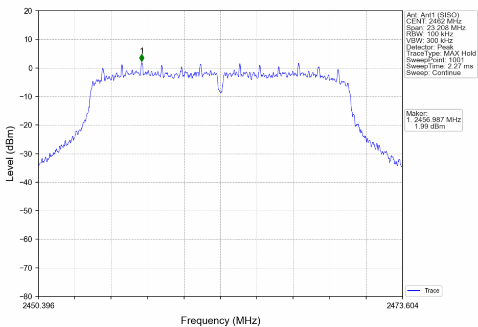
802.11g_HCH_2462MHz_Ant1 (SISO) NTN
