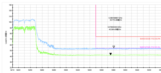
802.11ac VHT40-Channel 46: Peak + Average
