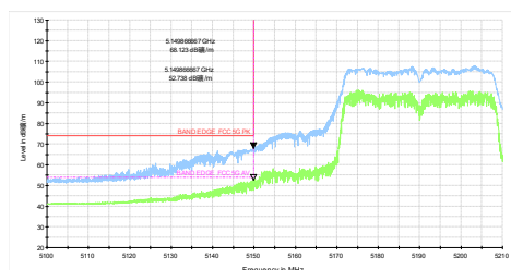
802.11ac VHT80 -Channel 42: Peak + Average
