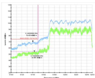
802.11ac VHT80 -Channel 42: Peak + Average
