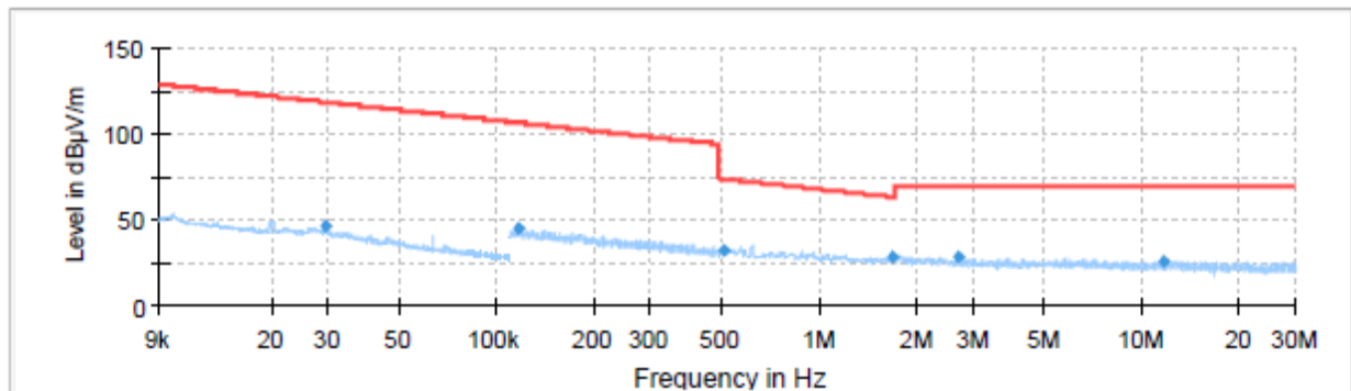
Radiates Emission from 9kHz-30MHz
