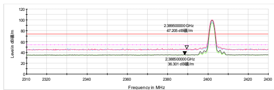
Bluetooth LE Channel 0 Peak+ Average
