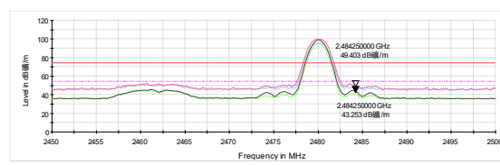
Bluetooth LE Channel 39 Peak+Average
