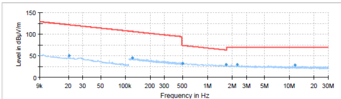
Radiates Emission from 9kHz-30MHz
