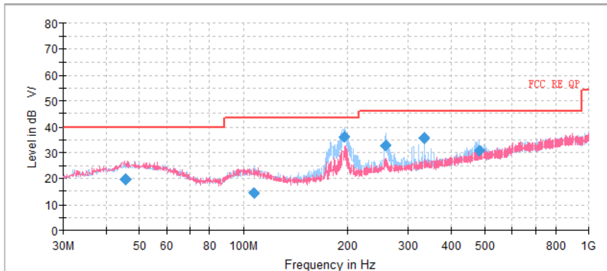
Radiates Emission from 30MHz to 1GHz
