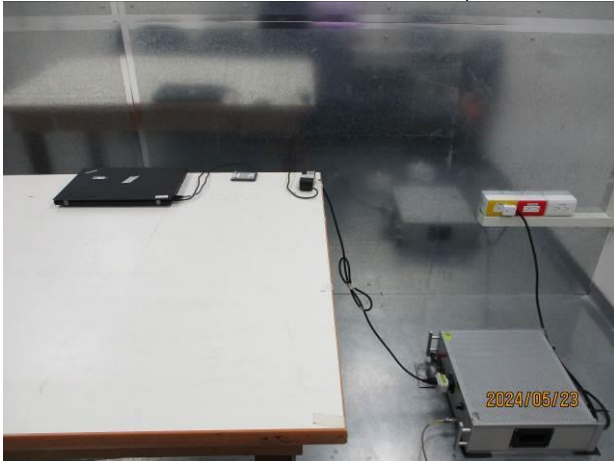
Part_15.225_NFC_Conduction_Setup
