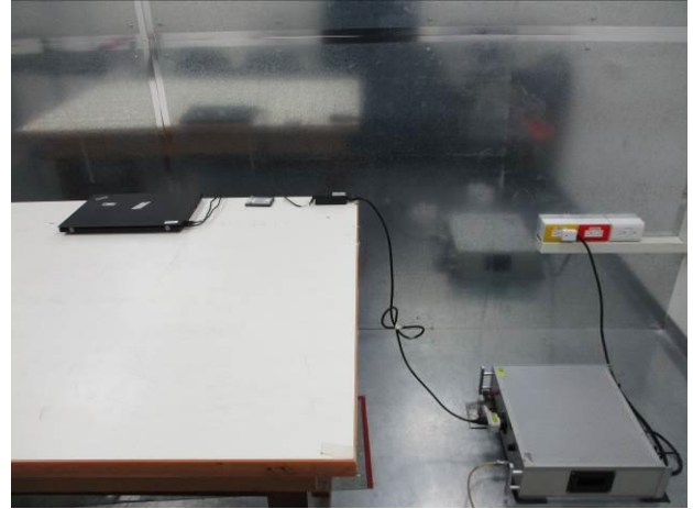
Part_15.247_BLE_Conduction_Setup
