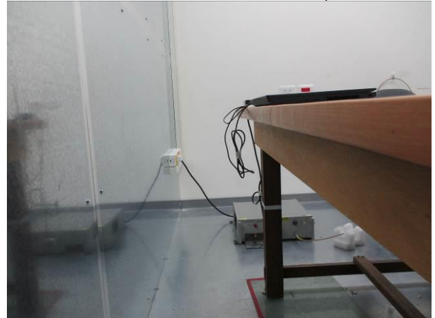
Part_15.247_BLE_Conduction_Setup
