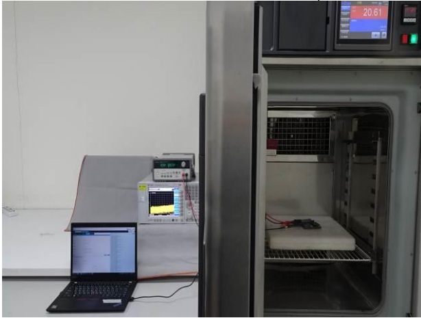
Part_15.247_BLE_Conducted_Setup
