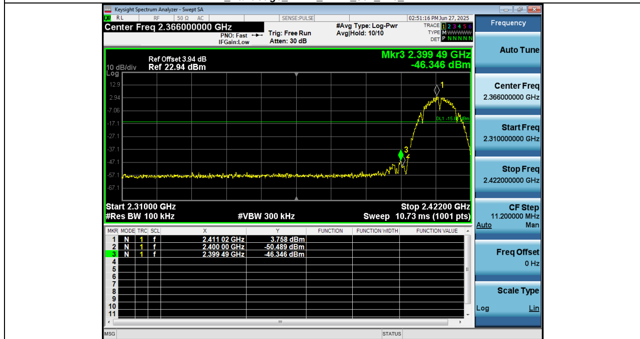
2_Bandedge_NVNT_ANT1_802_11b_2412
