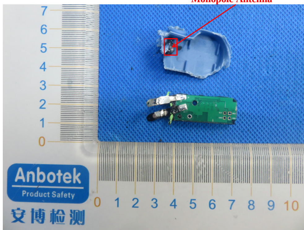
Monopole Antenna
