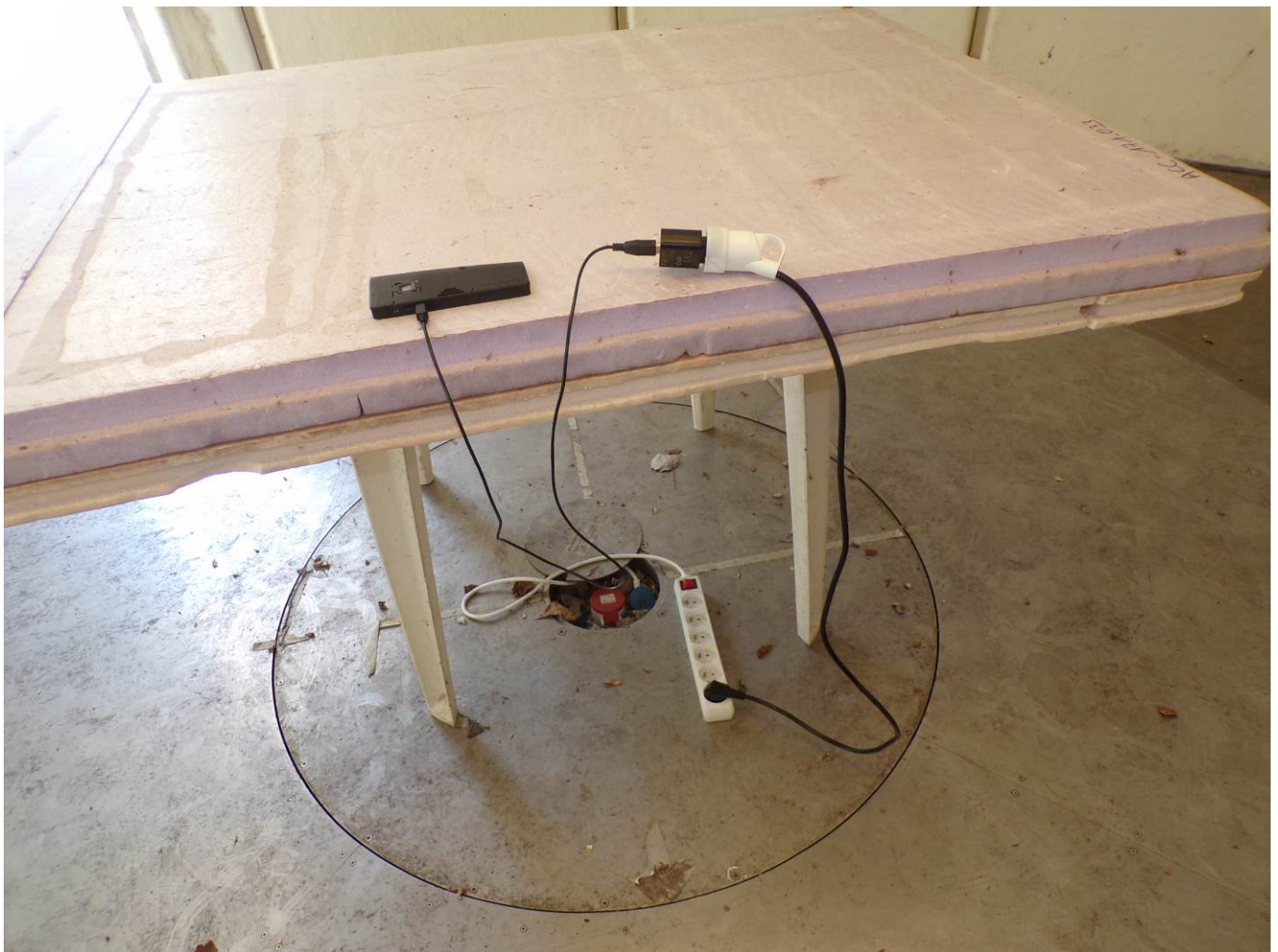
Open Area Test site (30M-1GHz, charging mode)
