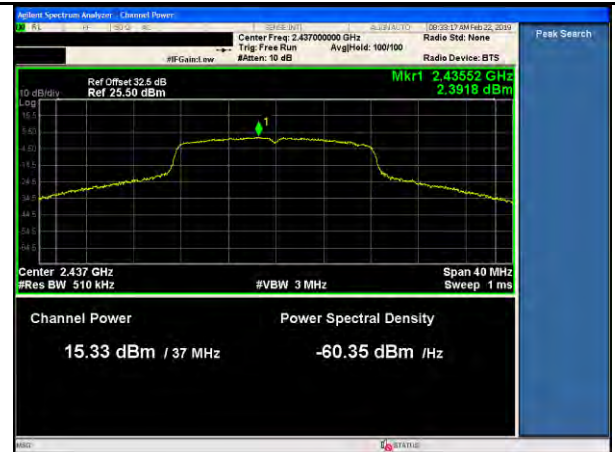
11g-PWR-Mid-54Mbps
