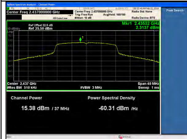
11g-PWR-Mid-6Mbps
