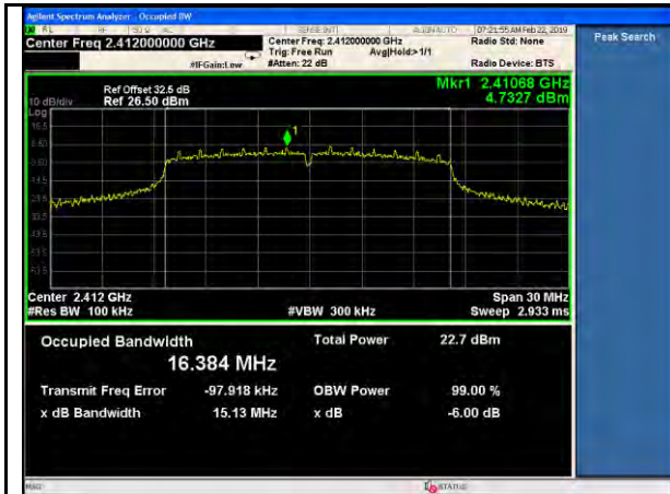
11g-6dB BW-Low-6Mbps
