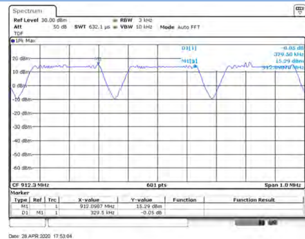
LoRa (250KHz)
