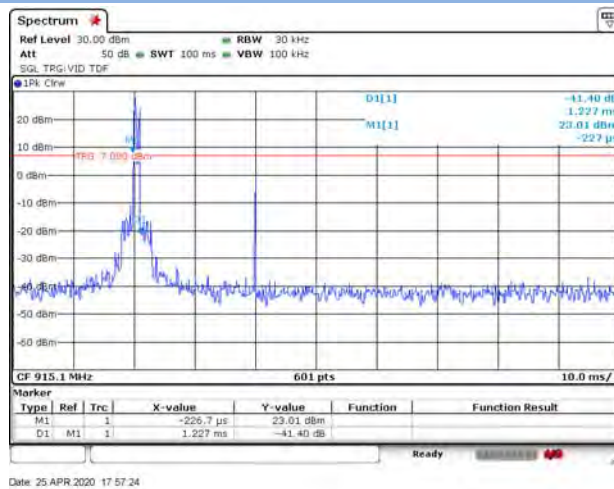
LoRa (125KHz)
