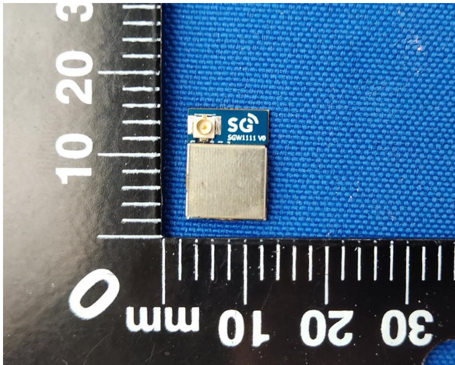
TOP VIEW OF EUT
