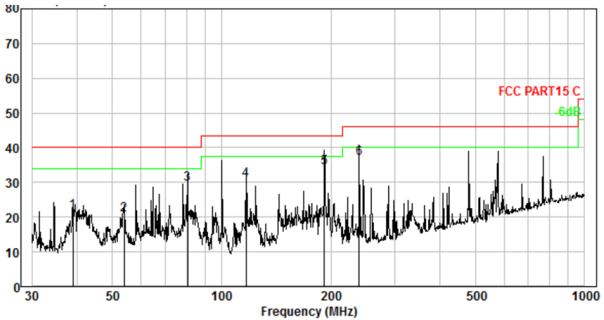
Test plot for Vertical: GFSK(2402MHz)
