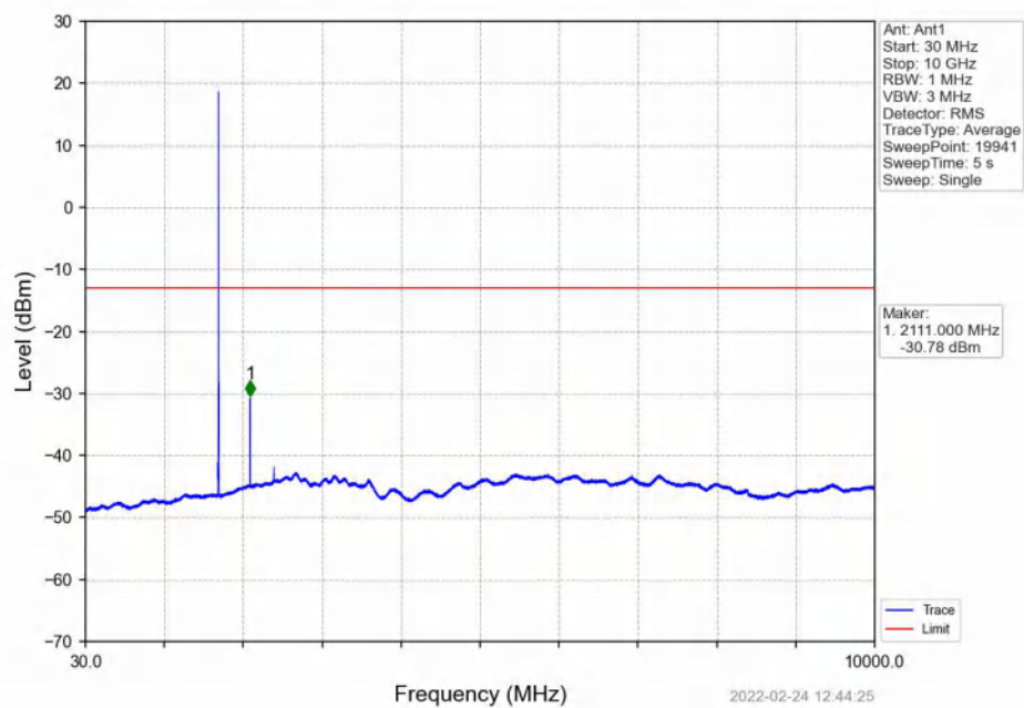
Band4_3MHz_16QAM_LCH_1711.5MHz_RB_1_0_NTNV
