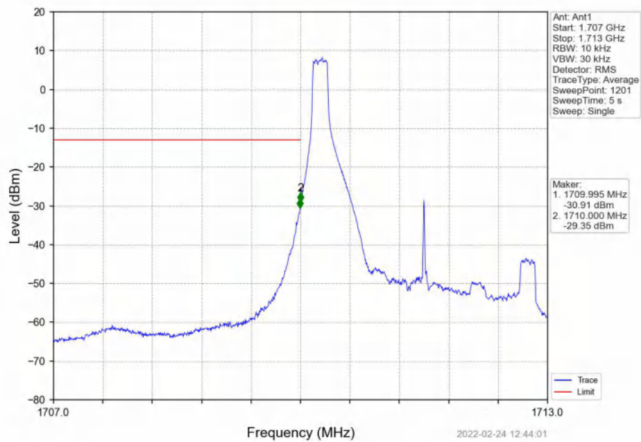
Band4_3MHz_16QAM_LCH_1711.5MHz_RB_1_0_NTNV
