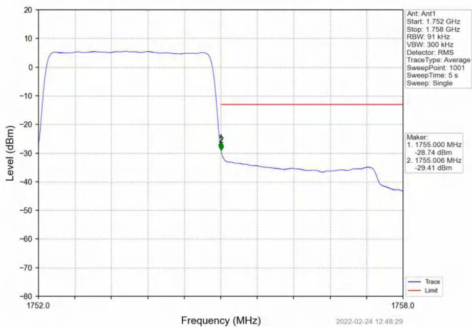
Band4_3MHz_QPSK_HCH_1753.5MHz_RB_15_0_NTNV
