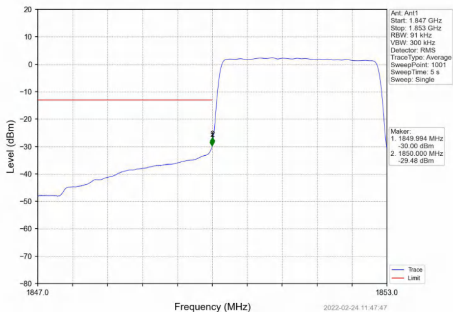
Band2_3MHz_QPSK_LCH_1851.5MHz_RB_15_0_NTNV
