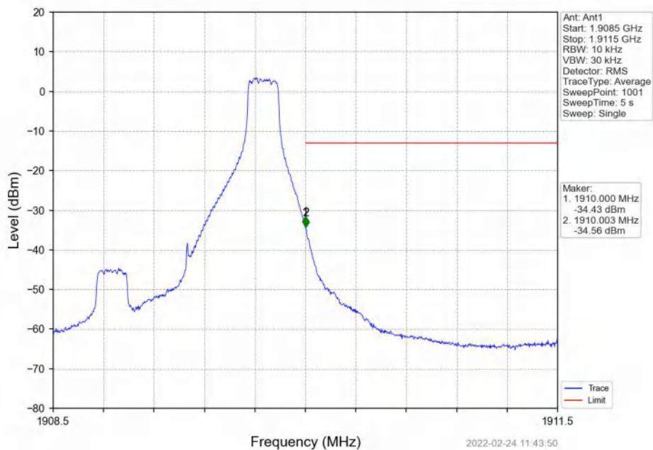
Band2_1.4MHz_QPSK_HCH_1909.3MHz_RB_6_0_NTNV
