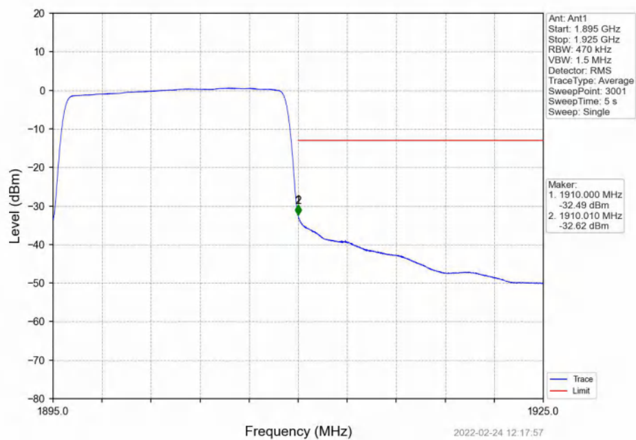
Band2_15MHz_QPSK_HCH_1902.5MHz_RB_75_0_NTNV
