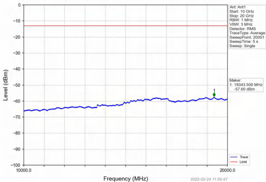
Band2_5MHz_QPSK_LCH_1852.5MHz_RB_25_0_NTNV
