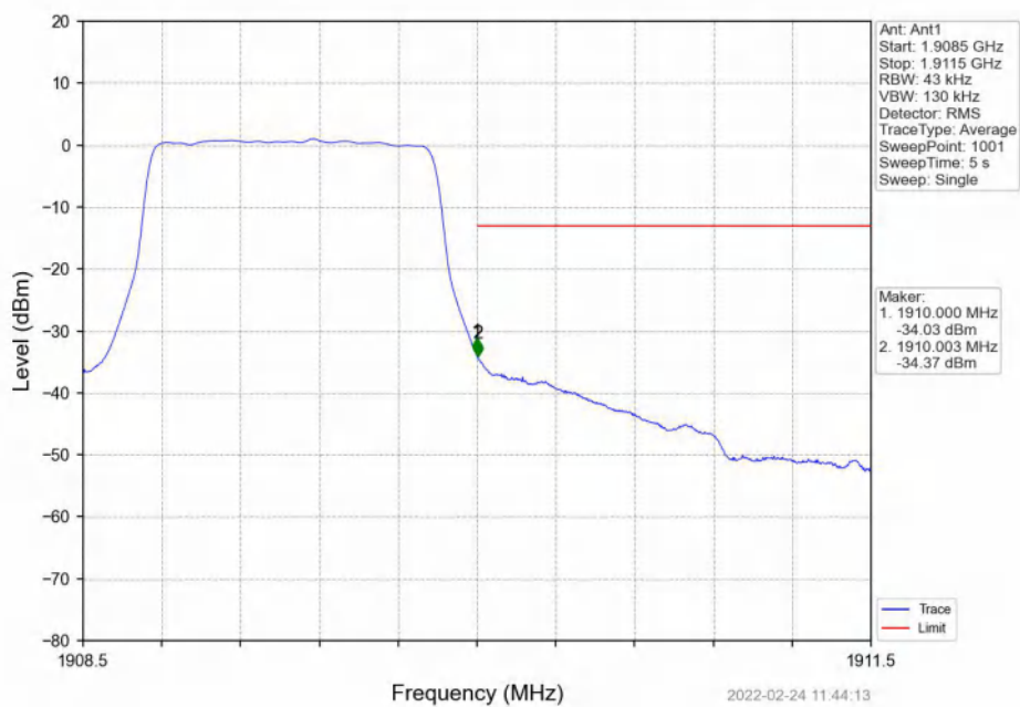
Band2_1.4MHz_QPSK_HCH_1909.3MHz_RB_6_0_NTNV
