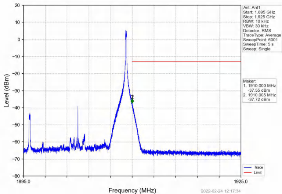
Band2_15MHz_QPSK_HCH_1902.5MHz_RB_75_0_NTNV
