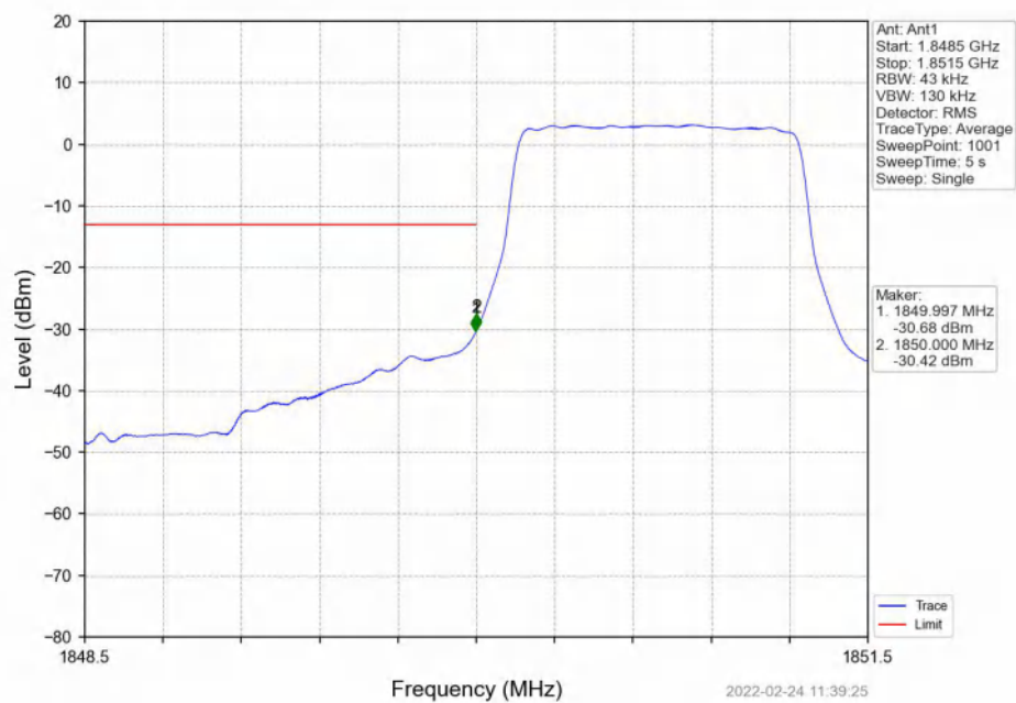
Band2_1.4MHz_QPSK_LCH_1850.7MHz_RB_6_0_NTNV
