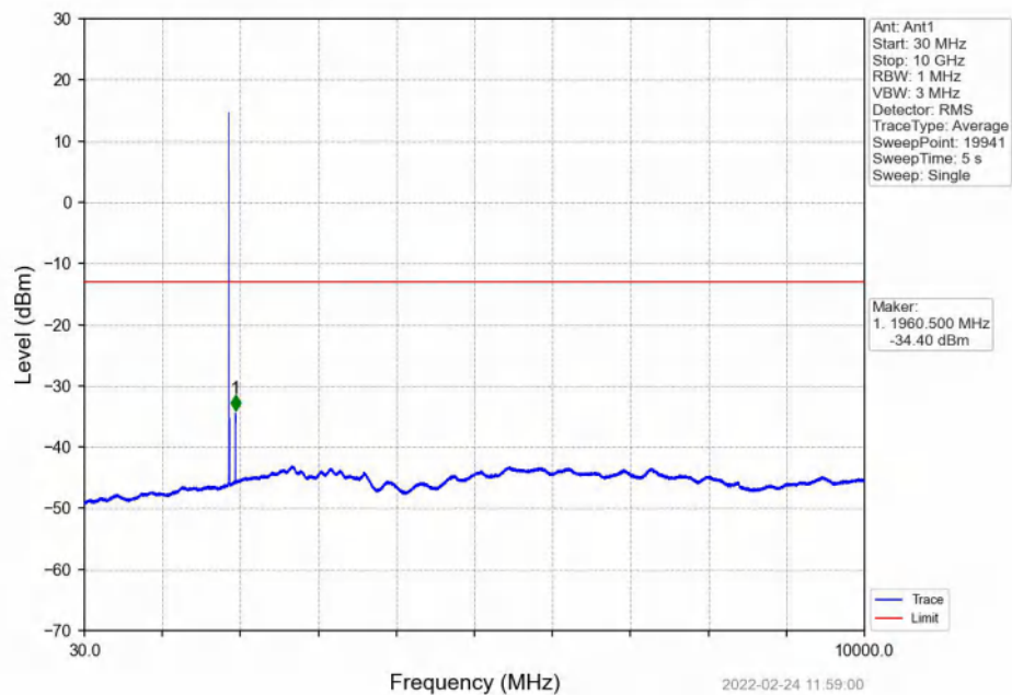
Band2_5MHz_16QAM_MCH_1880MHz_RB_1_0_NTNV
