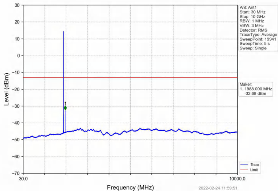
Band2_5MHz_QPSK_HCH_1907.5MHz_RB_1_0_NTNV
