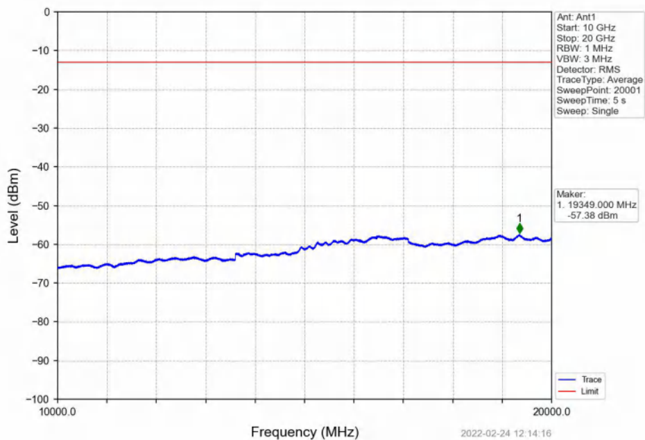
Band2_15MHz_16QAM_LCH_1857.5MHz_RB_75_0_NTNV
