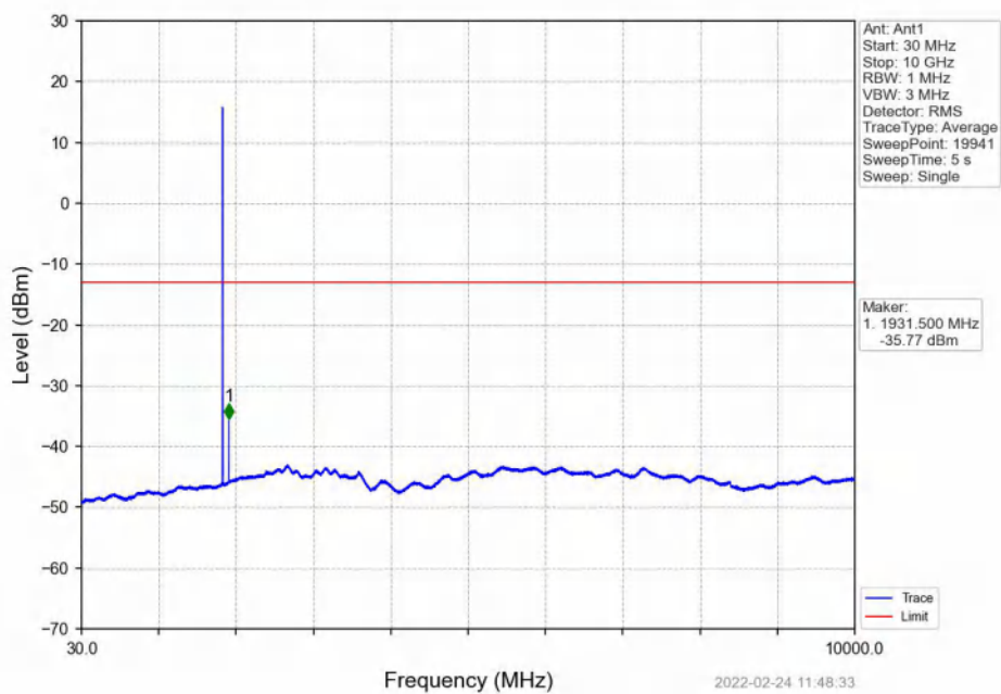
Band2_3MHz_16QAM_LCH_1851.5MHz_RB_1_0_NTNV
