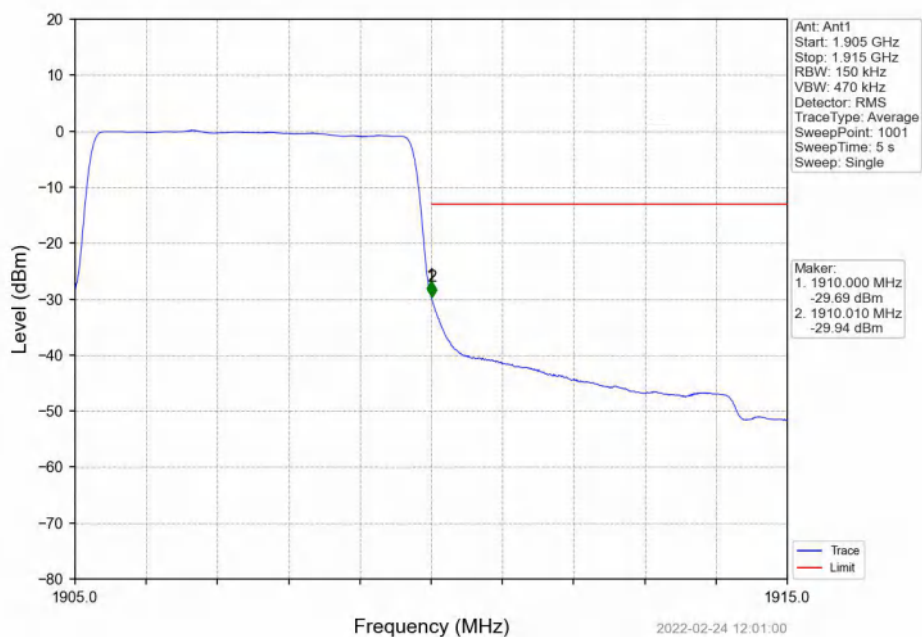
Band2_5MHz_QPSK_HCH_1907.5MHz_RB_25_0_NTNV
