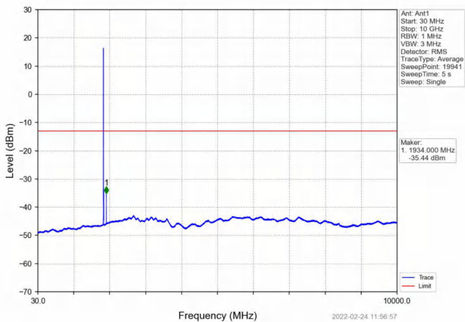
Band2_5MHz_16QAM_LCH_1852.5MHz_RB_1_0_NTNV
