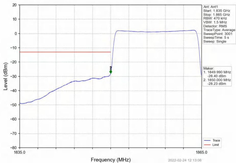
Band2_15MHz_QPSK_LCH_1857.5MHz_RB_75_0_NTNV
