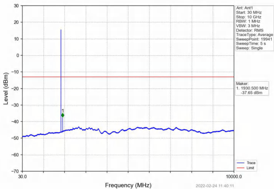
Band2_1.4MHz_16QAM_LCH_1850.7MHz_RB_1_0_NTNV
