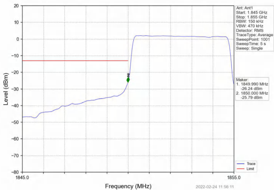
Band2_5MHz_QPSK_LCH_1852.5MHz_RB_25_0_NTNV
