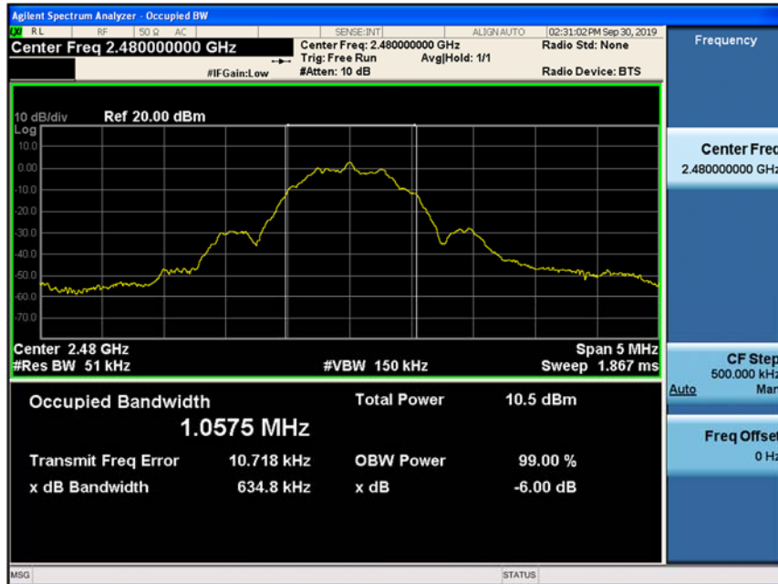
99% Bandwidth plot (High-CH 39)
