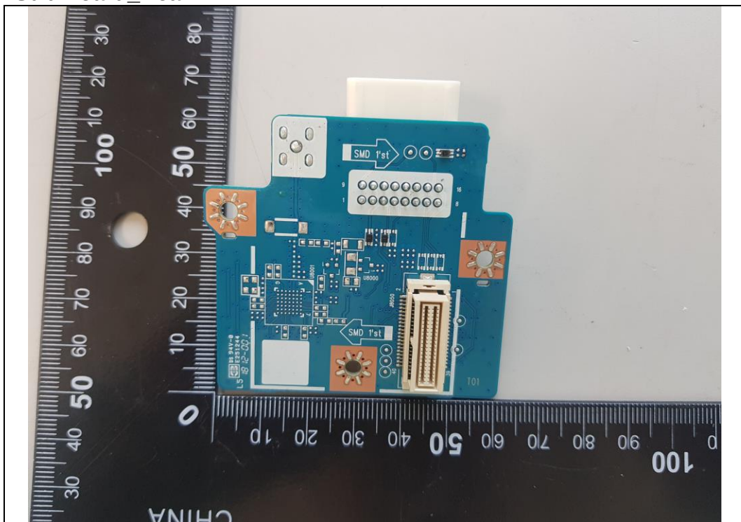
Sub Board_Rear
