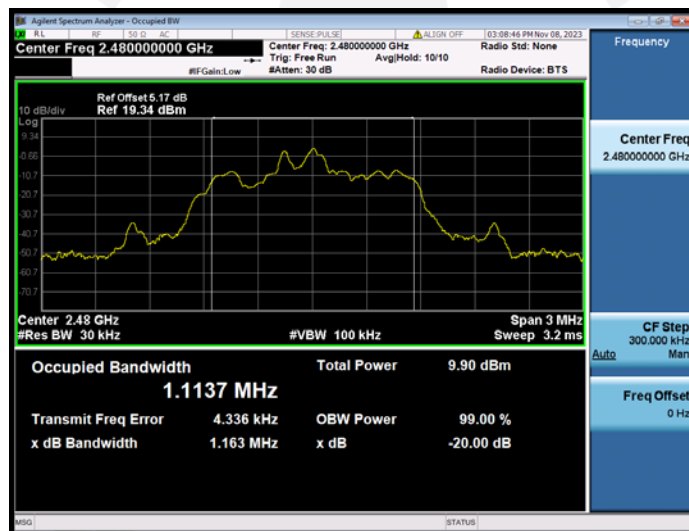
8DPSK (3-DH1) 2480MHz
