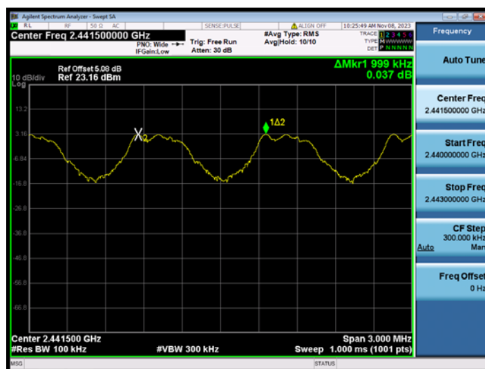
GFSK (1-DH1) 2441MHz
