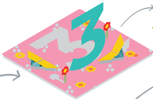
Flapping Butterfly
