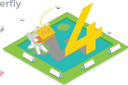
Talking Frog
