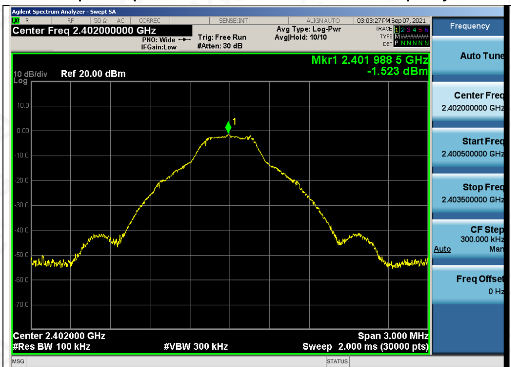
Test_Graph_BR_ANT1_2402_1Mbps_Reference Level
