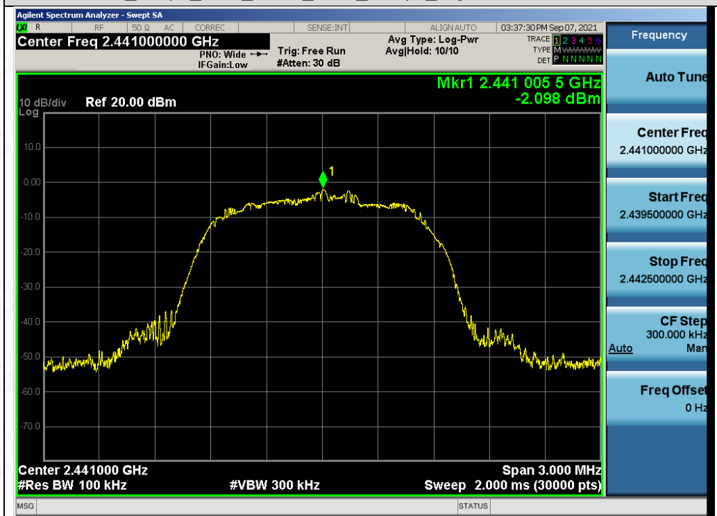
Test_Graph_EDR_ANT1_2441_3Mbps_Reference Level
